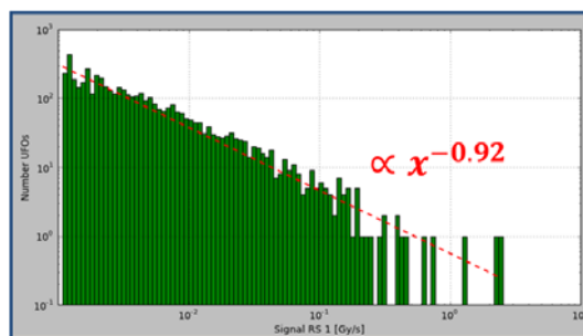
(a) Distribution of peak signal of UFO events.
