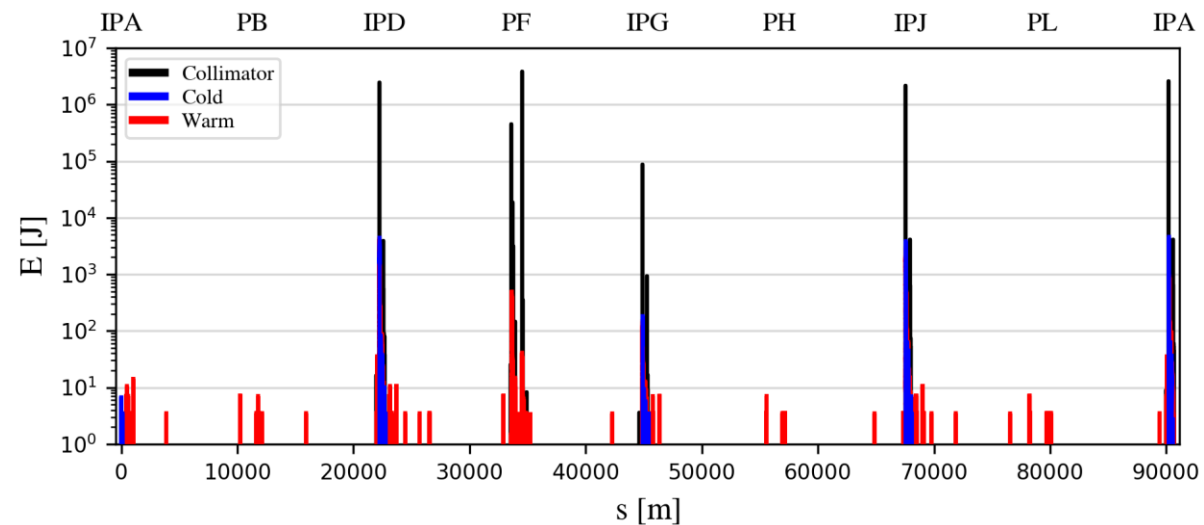
90deg phase
