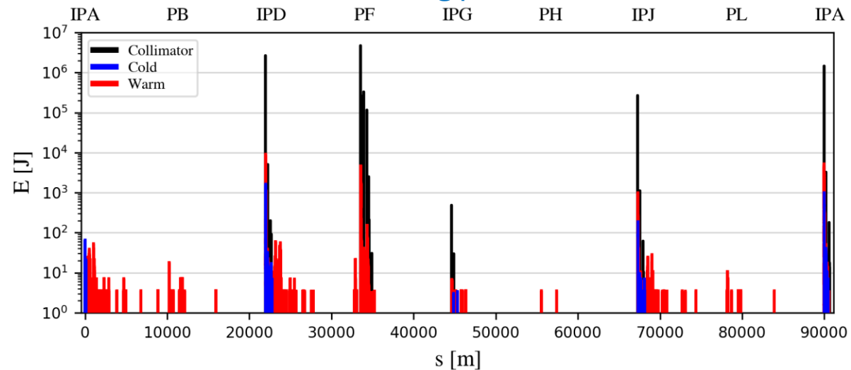
30deg phase
