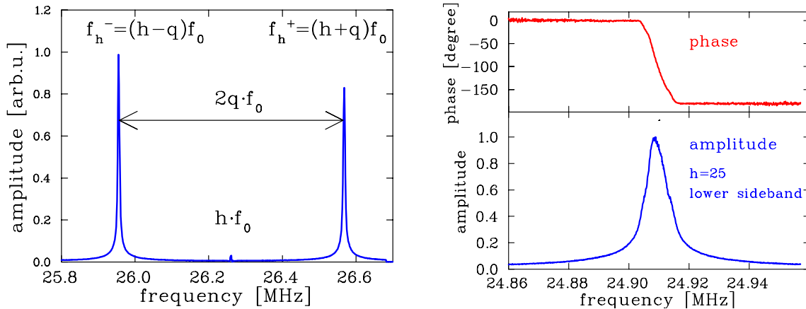
Figure 5.32: BTF measurement at the GSI synchrotron with a 500 MeV/u U^{73+} beam having a revolution frequency of f_0 = 1.048 MHz. The wide scan around the h = 25^{th} -harmonics is shown left and a scan around the lower sideband centered at f_{25}^- on the right. The fractional tune is q = 0.306 for these data.
