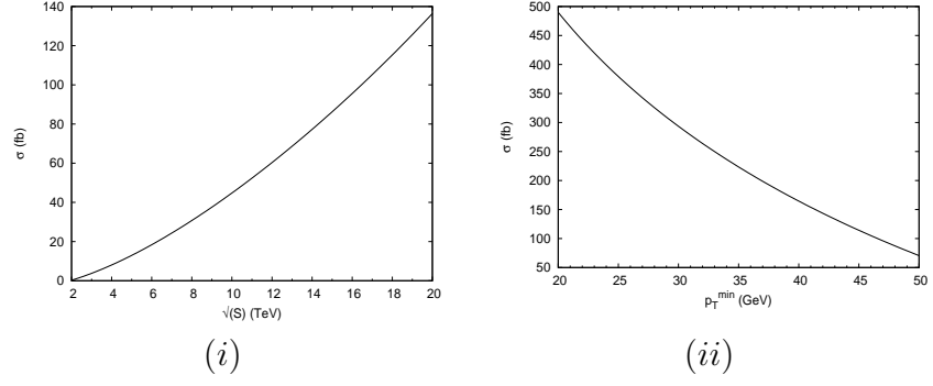
Figure 2: (i) Centre of mass energy (ii) p_T^{min} dependence of the cross section (at 14 TeV) for gg \rightarrow \gamma Zg .
