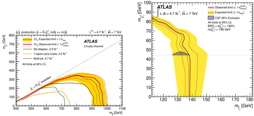
Figure 2: Exclusion limits in a gluino-mediated \tilde{t} [9] (left) and a direct \tilde{t} with \tilde{t} \rightarrow b\tilde{\chi}_{1,2}^{\pm} [12] (right) model.
