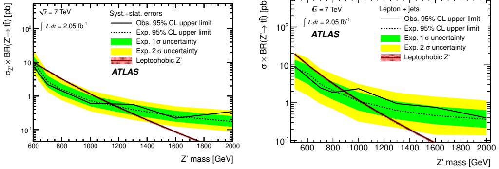
Figure 3: Comparison of exclusion limits in a leptophobic Z' model using the boosted (left) [23] and resolved (right) [24] t\bar{t} resonance searches.
