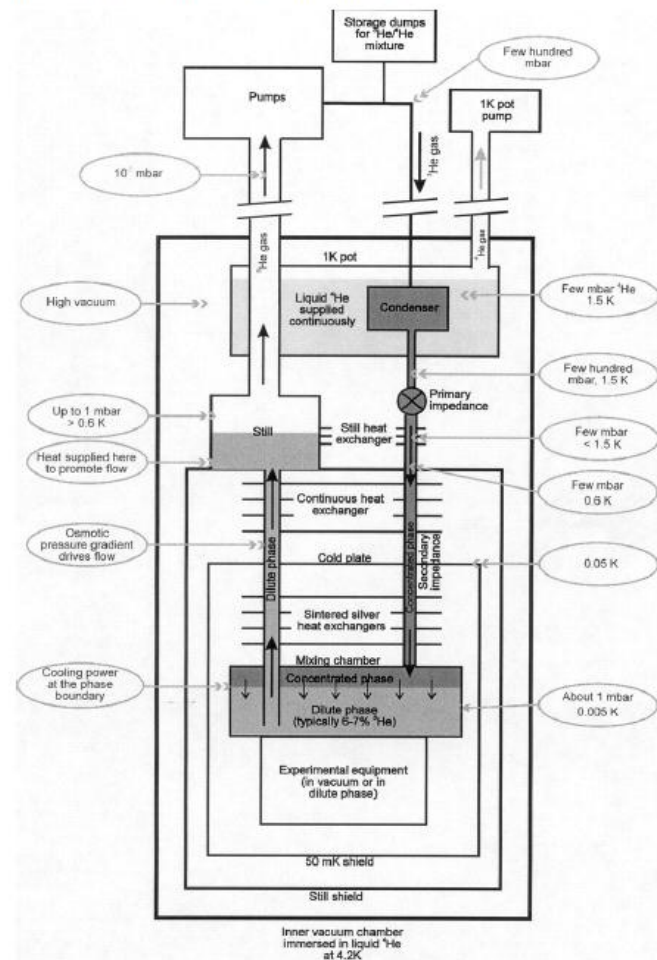
Fig. 9: Schematic diagram of dilution refrigerator
