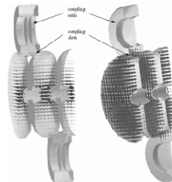
Side Coupled Structure (SCS)
