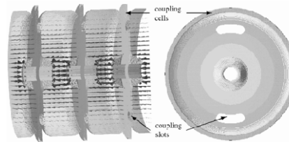
Side Coupled Structure (SCS)
