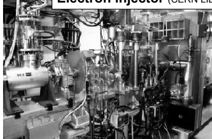
Electron injector (CERN LIL)
