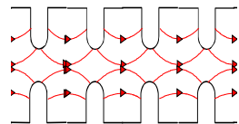
Disc-loaded structures operating in 0-mode
