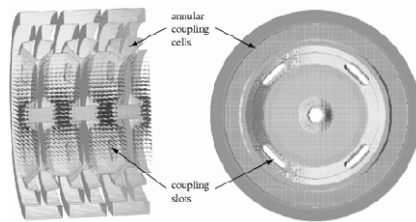
Annular ring Coupled Structure (ACS)
