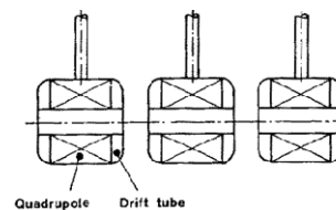
Maximize coupling between cells → remove completely the walls
