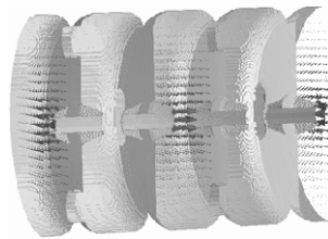
Annular ring Coupled Structure (ACS)
