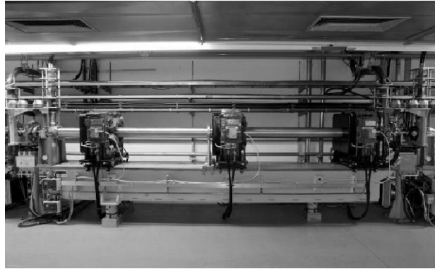
A 3 GHz LIL accelerating structure used for CTF3. It is 4.5 meters long and provides an energy gain of 45 MeV. One can see 3 quadrupoles around the RF structure.
