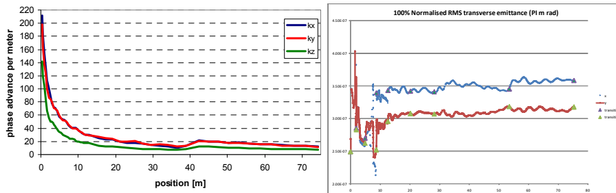
Transverse r.m.s. emittance and phase advance along Linac4 (RFQ-DTL-CCDTL-PIMS)
