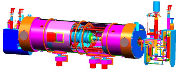
Figure 6: Medium Beta Cut-Away
