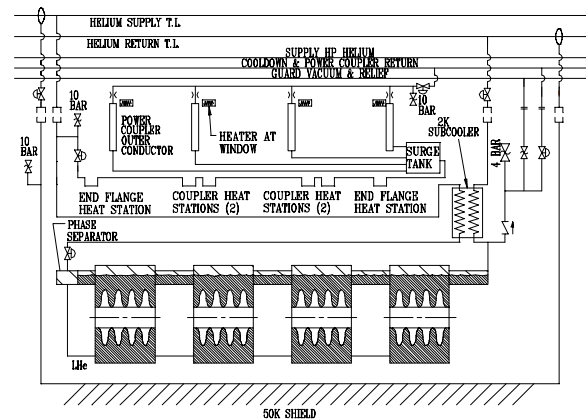
Figure 2: Flow Schematic
