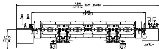
Figure 1: High Beta Cryomodule
