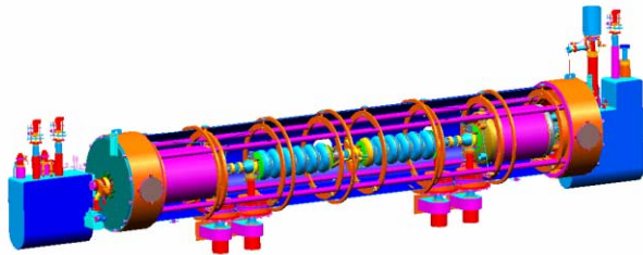
Figure 5: High Beta Cut-Away
