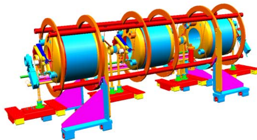
Figure 4: Cavity String Components Inside the Spaceframe Situated on Tooling
