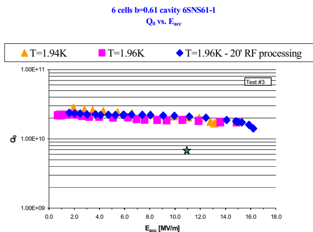
Figure 3: Medium Beta Cavity Performance
