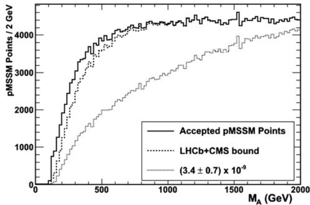
Fig. 9 Distribution of pMSSM points after the B_s^0 \rightarrow \mu^+ \mu^- constraint projected on the M_A (left) and (M_A, \tan \beta) plane (right) for all accepted pMSSM points (medium grey), points not excluded by the combination of the 2010 LHCb and CMS analyses (dark grey) and the
