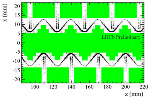
Fig. 30 Left: Distribution in x and z , for |y| < 1 mm, of the reconstructed vertices. The visible structures reflect the geometry of the vertex detector, with the pairs of silicon sensors appearing as pairs of vertical bands and the corrugated (“RF”) foil as the two wave shapes. The green shaded region represents the fiducial vacuum volume in which candidates are accepted. Right: Flight distance of offline reconstructed
