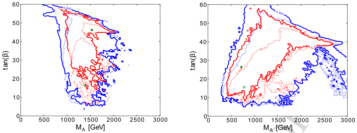
Fig. 8 Impact of the latest B_s^0 \rightarrow \mu^+ \mu^- limits on the (M_A, \tan \beta) plane in the (left) CMSSM and (right) NUHM1 [168]. In each case, the full global fit is represented by an open green star and dashed blue
