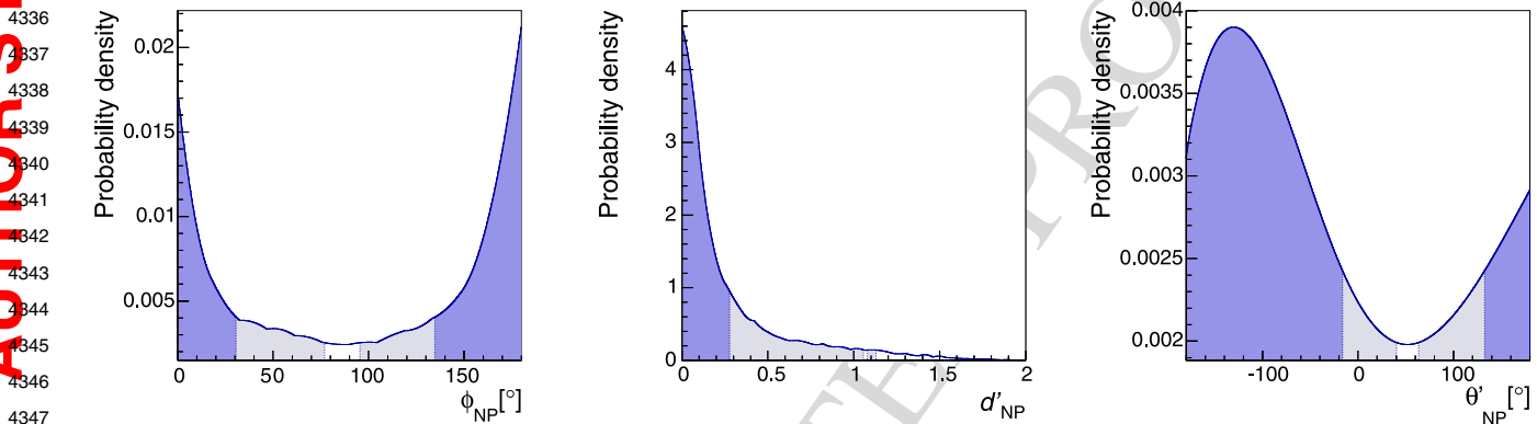
Fig. 22 From left to right: PDFs for \phi_{NP} , d'_{NP} and \theta'_{NP} obtained using the combined method with \kappa = 0.5 [357]
