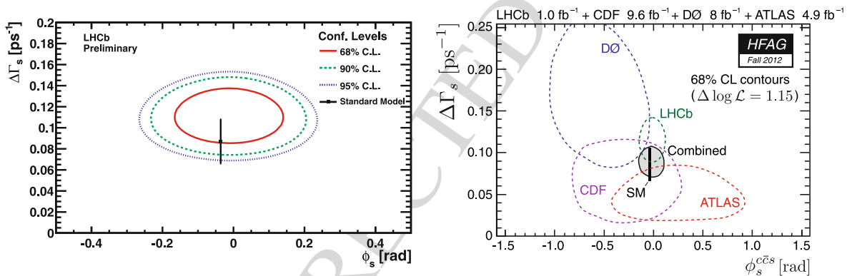
Fig. 10 (Left) Preliminary LHCb measurement of \phi_s and \Delta \Gamma_s from B_s^0 \rightarrow J/\psi \phi decays using 1.0 fb ^{-1} [139]. (Right) HFAG 2012 combination of \phi_s and \Delta \Gamma_s results, where the 1 \sigma confidence region is shown for each experiment and the combined result [44]. Note the different scales
