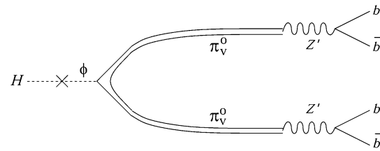
7399 7400 7401 7402 7403 7404 7405 7406 Fig. 29 Decay of a Higgs via a scalar field \phi into two \pi_v^0 particles, 7407 with \pi_v^0 charge equal to zero, which subsequently decay into b\bar{b} jets. (Adapted from Ref. [601])
