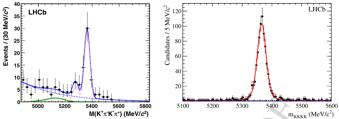
Fig. 15 (Left) fit of the K^+\pi^-K^-\pi^+ mass distribution for B_s^0 \rightarrow K^{*0}\bar{K}^{*0} candidates from 35 \text{ pb}^{-1} [303]; (right) fit of the K^+K^-K^-K^+ mass distribution for B_s^0 \rightarrow \phi\phi candidates from 1.0 \text{ fb}^{-1} [304]
