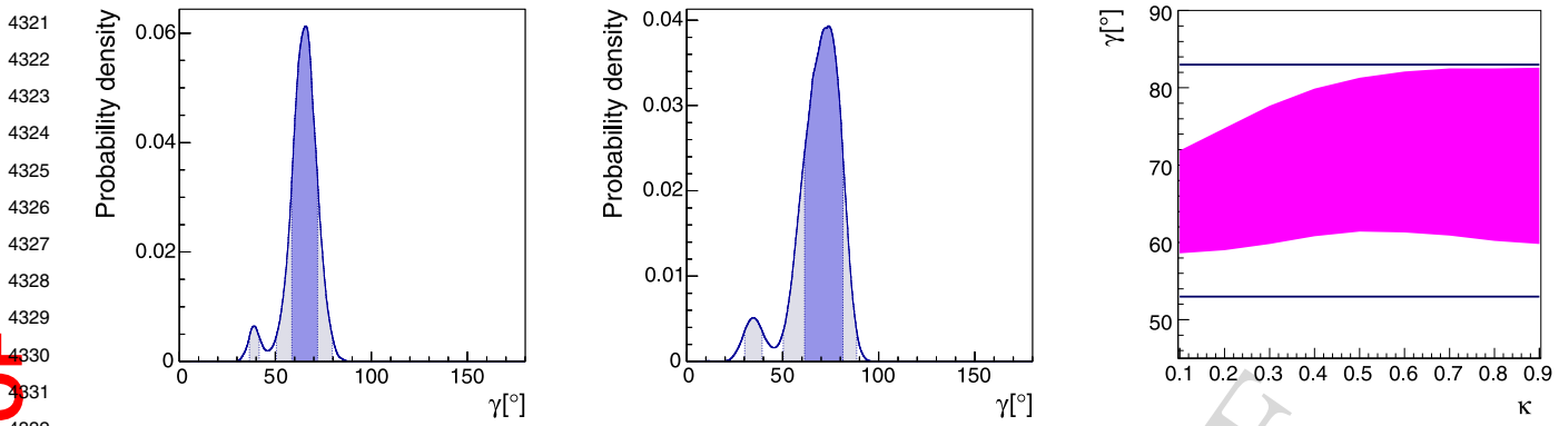
Fig. 21 From left to right: PDF for \gamma obtained using the combined method for \kappa = 0.1, 0.5 ; 68 % probability region for \gamma obtained using the combined method (filled area) or the GL method (horizontal lines) as a function of \kappa [357]
