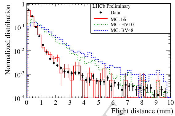
vertices in events outside the matter region. Data are compatible with b\bar{b} background. The black points are for data in 36 \text{ pb}^{-1} [605], the red line is a full simulation of b\bar{b} production and the green dashed line is a full simulation of the HV benchmark channel. The blue dashed line shows a simulation of a model with baryon number violating neutralino couplings
