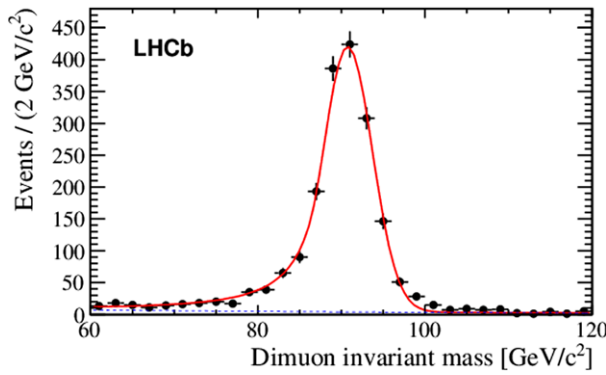
Fig. 28 LHCb Z and W production results from 37 \text{ pb}^{-1} at \sqrt{s} = 7 \text{ TeV} [588]. Left: Z \rightarrow \mu^+ \mu^- peak. Right: W^+ - W^- production asymmetry, where the bands correspond to the experimental uncertainties (only indicated within the LHCb acceptance), and the data points
