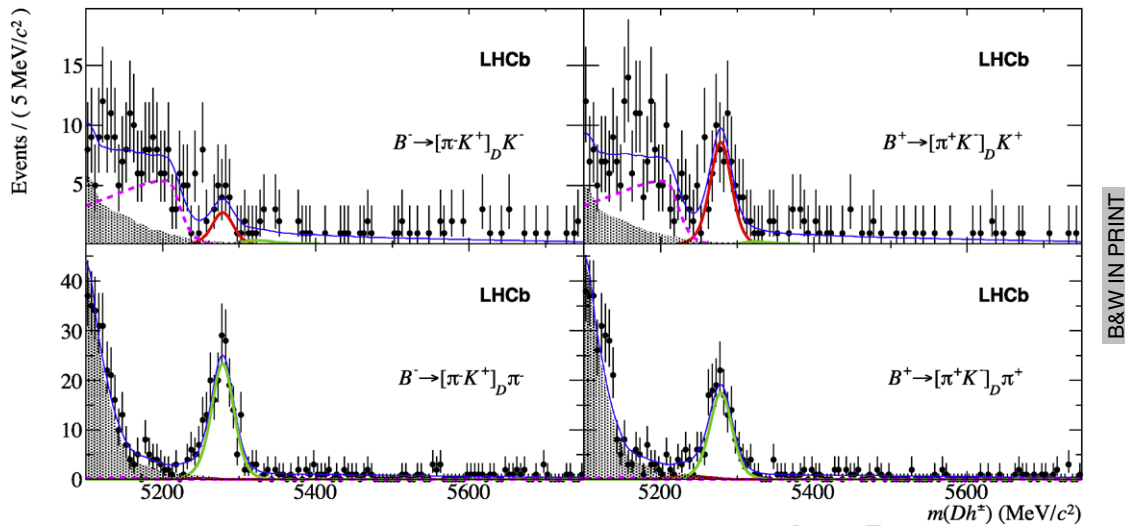
Fig. 18 Invariant mass distributions of selected B^\pm \rightarrow [\pi^\pm K^\pm]_D h^\pm candidate events: (left) B^- candidates, (right) B^+ candidates [6]. In the top plots, the track directly from the B vertex passes a kaon identification requirement and the B candidates are reconstructed assigning this track the kaon mass. The remaining events are placed in the bottom row and are reconstructed with a pion mass hypothesis. The dark
