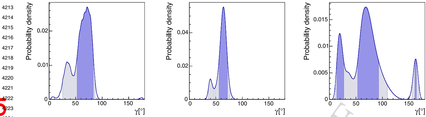
Fig. 20 From left to right: PDF for \gamma obtained using the GL method as described in the text; PDF for \gamma obtained using the Fleischer method for \kappa = 0.1, 0.5 [357]. Here and in the following, dark (light) areas correspond to 68 % (95 %) probability regions
