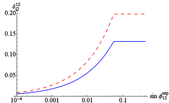
from the down sector is \lambda_C^5 (left panel) or \lambda_C^3 (right panel). The solid blue line in each panel is for \tilde{m}_{\tilde{Q}} = m_{\tilde{g}} = 1 TeV and the dashed red line is for \tilde{m}_{\tilde{Q}} = m_{\tilde{g}} = 1.5 TeV
