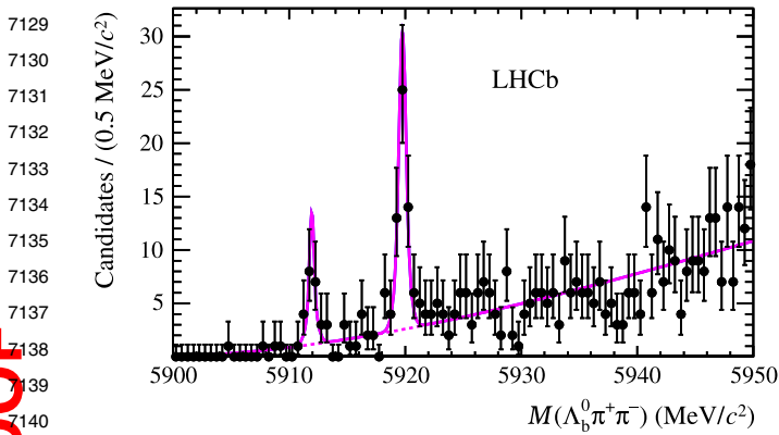
Fig. 27 Invariant mass spectrum of \Lambda_b^0 \pi^+ \pi^- [583]. The points with error bars are the data, the solid line is the result of a fit to this distribution, and the dashed line is the fitted background contribution
