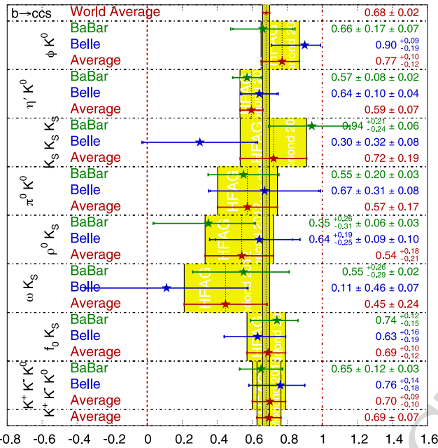
Fig. 16 HFAG compilation of results for \sin 2\beta^{\text{eff}} in b \rightarrow sq\bar{q} decays [44]
