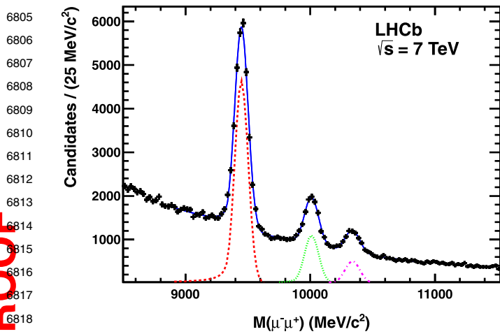
Fig. 25 Invariant mass distribution of selected \gamma candidates from 25 \text{ pb}^{-1} of data collected in 2010 [524]. The \gamma(1S) , \gamma(2S) and \gamma(3S) states are clearly resolved. The results of a maximum likelihood fit are superimposed
