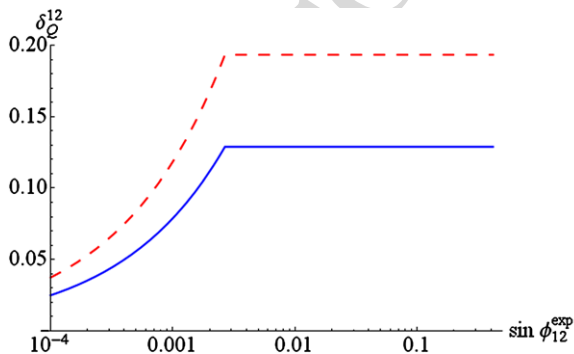
Fig. 24 Bound on the squark mass degeneracy \delta_Q^{12} , defined in Eq. (100), as a function of the experimental constraint on CP violation in D^0-\bar{D}^0 mixing, parametrised by \sin \phi_{12}^{\text{exp}} . The alignment angle
