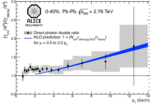
Figure 5: (color online) Direct-photon double ratio in Pb-Pb collisions at \sqrt{s_{\text{NN}}} = 2.76 \text{ TeV} for 0-40% centrality with NLO pQCD predictions
