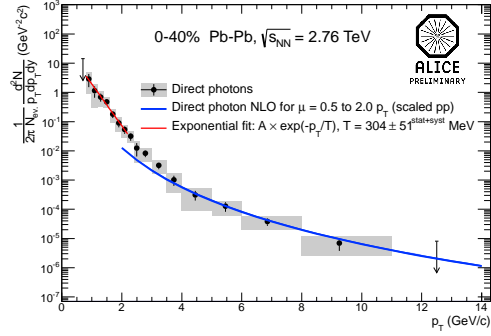
Figure 6: (color online) Direct-photon invariant yield in Pb-Pb collisions at \sqrt{s_{\text{NN}}} = 2.76 \text{ TeV} for 0-40% centrality with NLO pQCD predictions and exponential fit
