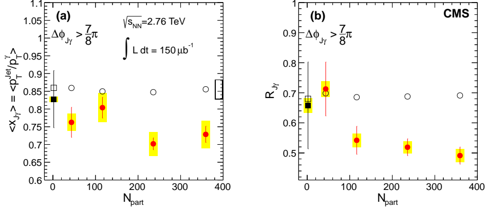
Figure 3: (a) Average ratio of jet transverse momentum to photon transverse momentum, \langle x_{J\gamma} \rangle , as a function of N_{\text{part}} . The empty box at the far right indicates the correlated systematic uncertainty. (b) Average fraction of isolated photons with an associated jet above 30 GeV/c, R_{J\gamma} , as a function of N_{\text{part}} . In both panels, the yellow boxes indicate point-to-point systematic uncertainties and the error bars denote the statistical uncertainty.
