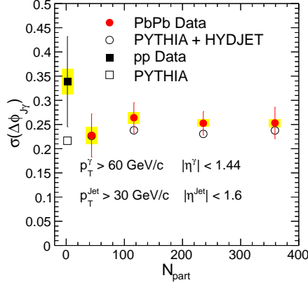
Figure 1: Fitted \Delta\phi_{J\gamma} width ( \sigma in Eq. (1), \Delta\phi_{J\gamma} > \frac{2}{3}\pi ) between the photon and associated jet after background subtraction as a function of N_{\text{part}} . The error bars show the statistical uncertainty, and the yellow boxes indicate the systematic uncertainties.
