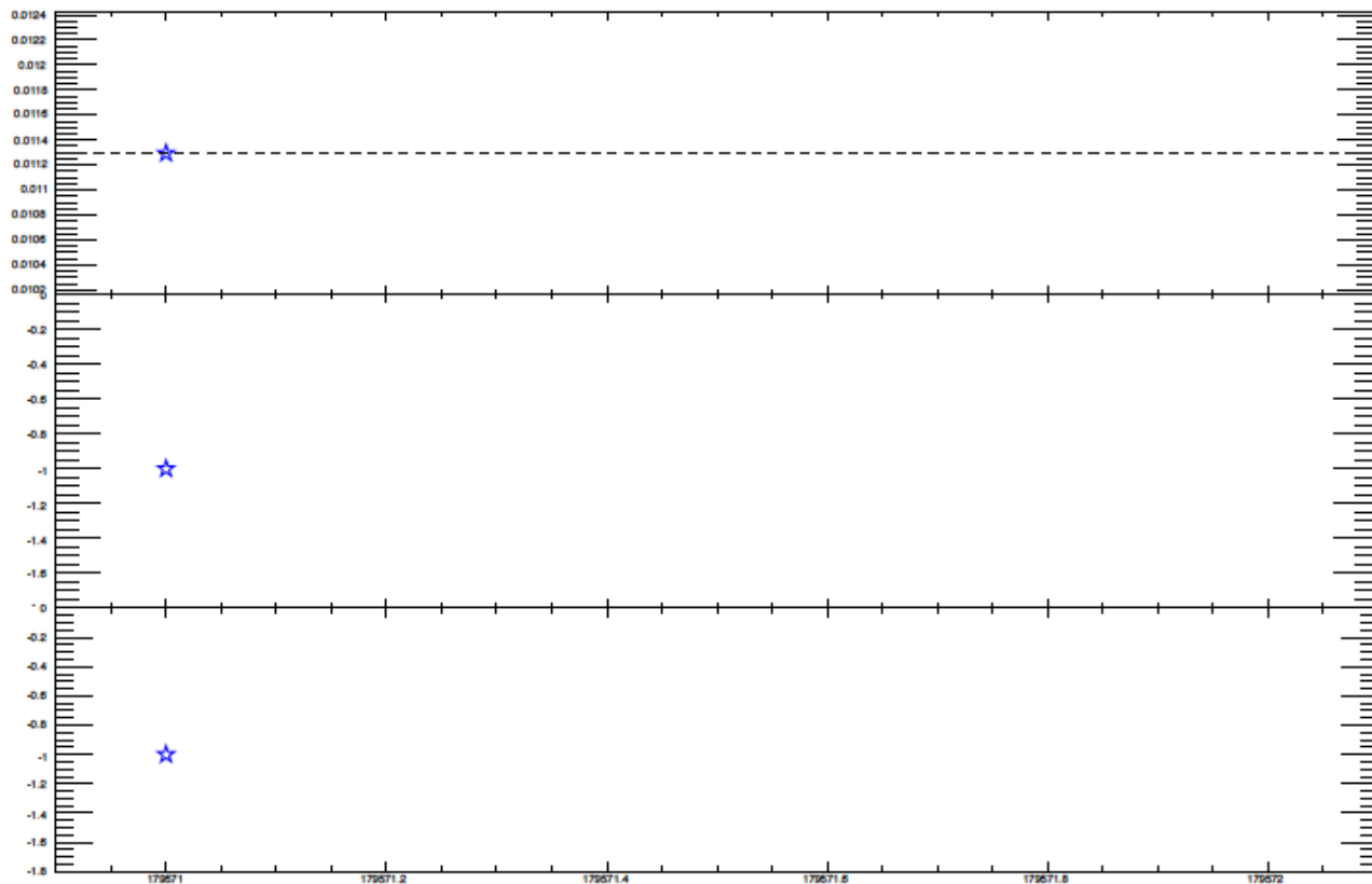
Tracklets vs Clusters BG Over All, LHC12_Test_cpas1, for kINT7 (top), kINT8 (mid), kMB (bottom)
