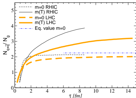
Figure 3. Quark plus anti-quark to gluon ratio as a function of \tau at RHIC (black thin lines) and at LHC (light thick lines). Dashed lines are for the massless case and the solid for the massive case.
