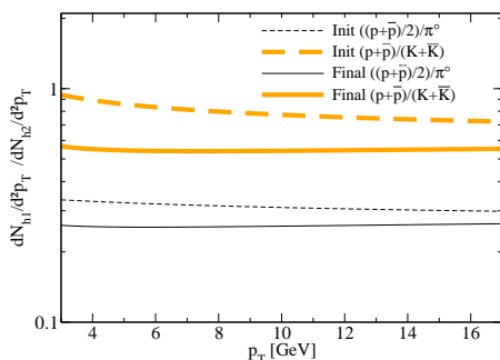
Figure 5. Ratio of hadrons obtained with the AKK fragmentation functions [10]. The dashed lines are the ratio according to the initial partons distributions, the solid lines are at the freeze-out considering the effect of the inelastic collisions.
