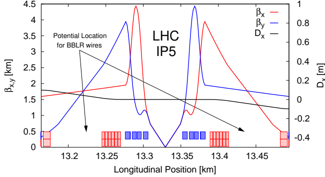
Figure 2: LHC interaction region schematically showing the common focusing channel with the 32 long-range interactions on the left and the right of the collision point (top) and the optics functions in the region.
