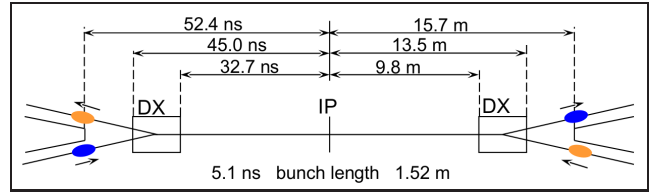
Figure 3: Schematic of the RHIC interaction regions.
