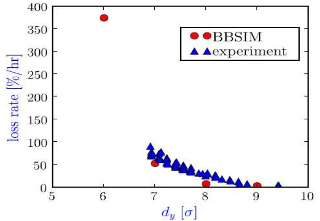
Figure 15: Comparison of measured and simulated beam loss rate as a function of distance between wire and beam. Experiment with gold beam at store, wire strength of 125 Am [56, 58].
