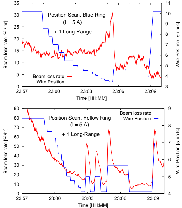
Figure 19: Beam loss rate for a Blue (top) and Yellow (bottom) bunch with one long-range interaction, and an additional wire interaction. The wire position varies, and the wire current is constant at 5 A.
