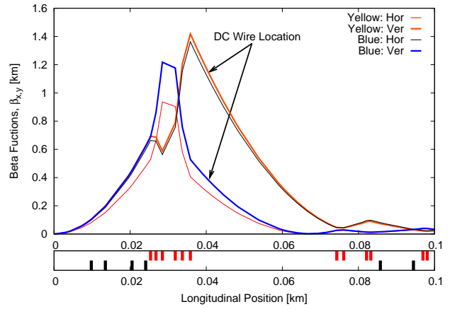
Figure 9: The beta functions from MAD lattice for both rings as a function of longitudinal position.
