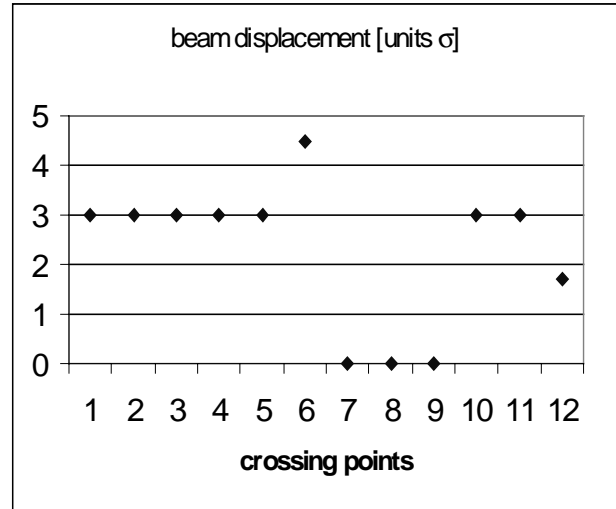
Fig 2 : beam half-separation in the 12 crossing points. .
