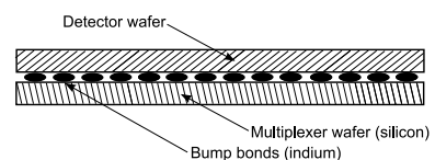
Fig. 3. SCUBA-2 detector and multiplexer bonding method.
