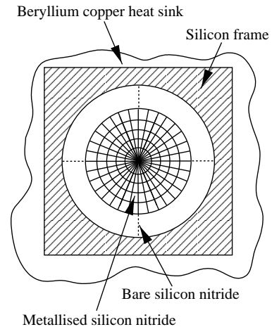
Fig. 2. Layout of a spiderweb bolometer.
