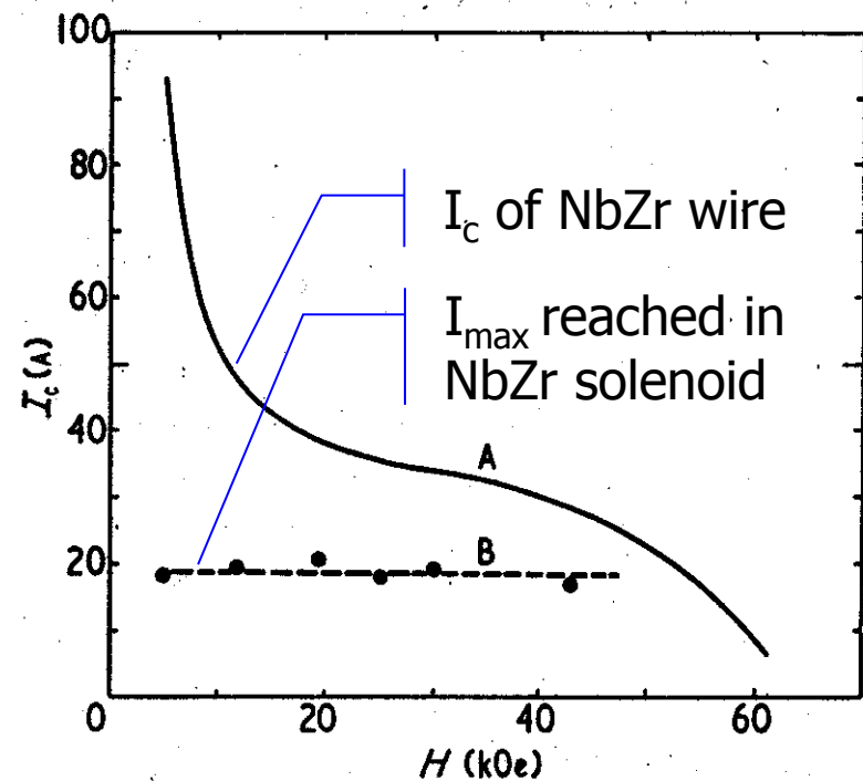
NbZr solenoid vs. wire Chester, 1967
