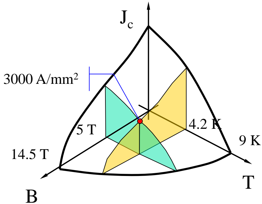
typical NbTi
