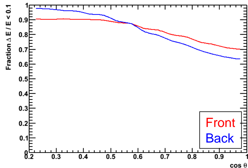
Containment within 10% of E_{\text{true}}
