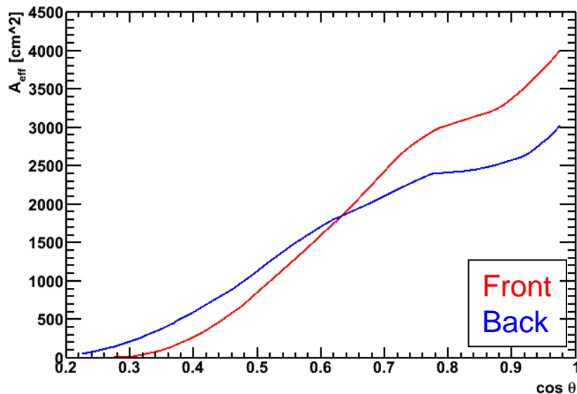
A_{\text{eff}}(\cos\theta) at 130GeV
