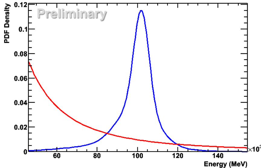
Signal and Bkg. PDFs
