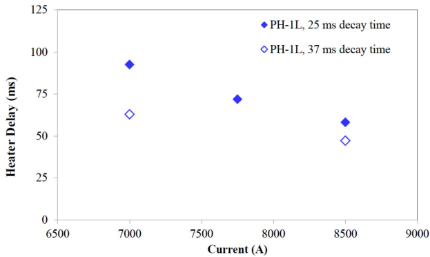
Fig. 14: Heater delay as a function of magnet current for the peak heater power of \sim 20 \text{ W/cm}^2 and different decay time constant of the heater circuit.
