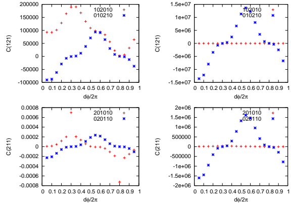
Figure 9: Coefficients of x y^2 z and x^2 y z terms of the beam-beam interaction. (a) x y^2 z (102010) and p_x p_y^2 z (010210) for the horizontal-horizontal crossing. (b) x y^2 z (102010) and p_x p_y^2 z (010210) for the horizontal-vertical crossing. (c) x^2 y z (201010) and p_x^2 p_y z (020110) for the horizontal-horizontal crossing. (d) x^2 y z (201010) and p_x^2 p_y z (020110) for the horizontal-vertical crossing.
