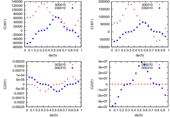
Figure 8: Coefficients of x^3 z and y^3 z terms of the beam-beam interaction. (a) x^3 z (300010) and p_x^3 z (030010) for the horizontal-horizontal crossing. (b) x^3 z (300010) and p_x^3 z (030010) for the horizontal-vertical crossing. (c) y^3 z (003010) and p_y^3 z (000310) for the horizontal-horizontal crossing. (d) y^3 z (003010) and p_y^3 z (000310) for the horizontal-vertical crossing.
