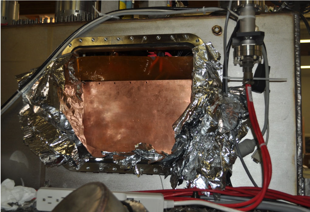
Access hatch open with copper shield plates in front of HTS leads
