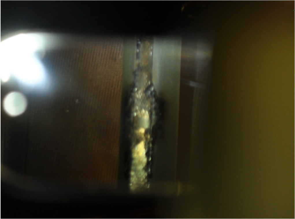
A portion of the front of the burned out lead (using a mirror)
