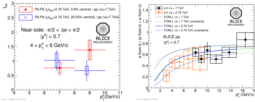
Figure 3: Yield modification in Pb-Pb relative to pp collisions (left panel). Relative beauty contribution to the total cross section of electrons from heavy-flavour decays, as a function of p_T , in pp collisions (right panel).
