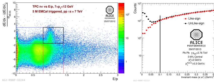
Figure 1: Electron identification using TPC and EMCal information (left panel). Invariant Mass of e^\pm e^\mp (black points) and e^\pm e^\pm (red points) pairs, used to reconstruct electrons from gamma conversions in the detector material and from light meson Dalitz decays (right panel).
