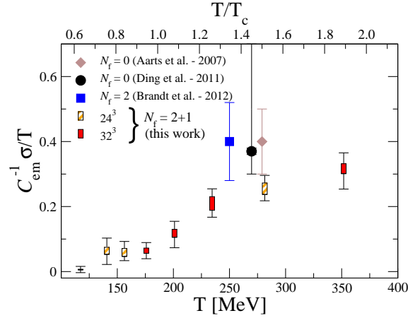
Figure 4. The conductivity, \sigma , as a function of temperature. As well as the results from our work, quenched ( N_f = 0 ) [18, 19] and dynamical results [20] are also shown.
