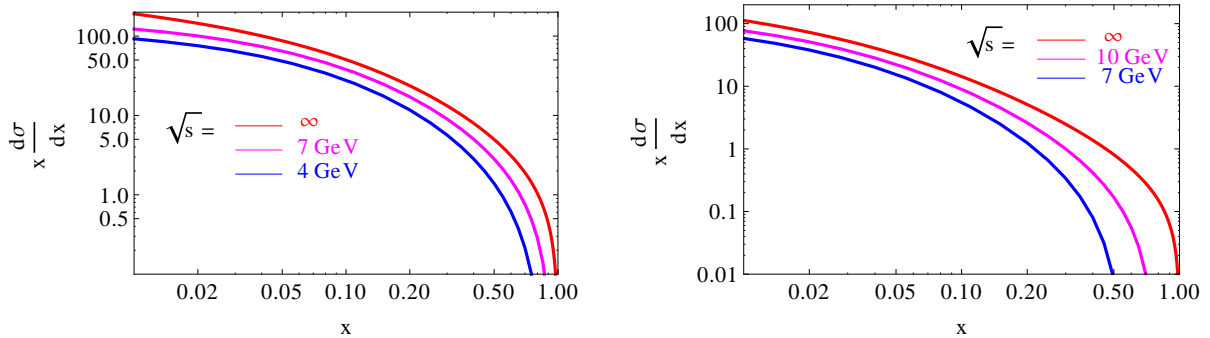
Figure 2. Charm (left) and bottom (right) fractional energy loss spectrum, x d\sigma/dx , for various \sqrt{s} , together with the high-energy approximation \sqrt{s} \rightarrow \infty . \mu = 0.4 GeV.
