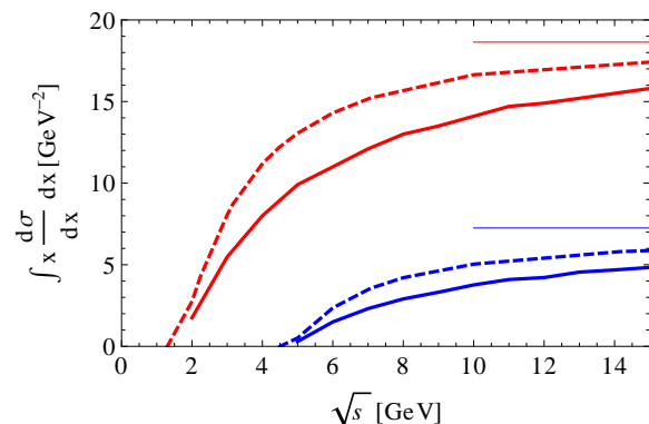
Figure 1. Energy dependence of \int x (d\sigma/dx) dx for charm (upper curves) and bottom (lower curves). Solid lines show the full energy dependence and dashed lines correspond to an approximation where the influence of finite energy is taken into account only in phase space boundaries. Thin straight lines show the asymptotic results. The screening scale is taken as \mu = 0.4 GeV.
