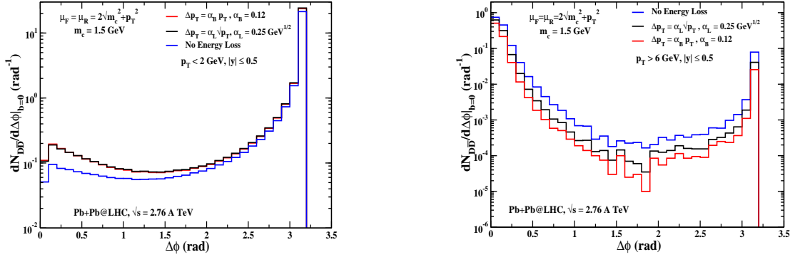
Figure 1. Effect of energy loss on azimuthal correlation of D\bar{D} pair for two different charm momentum region
