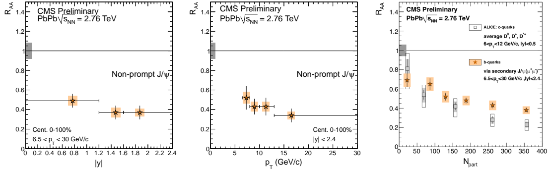
Figure 5. The non-prompt J/\psi R_{AA} with respect to rapidity ( left ), p_T ( center ) and centrality ( right ) are presented. Centrality dependence of open charm R_{AA} via D meson measurement by ALICE is compared to non-prompt J/\psi .
