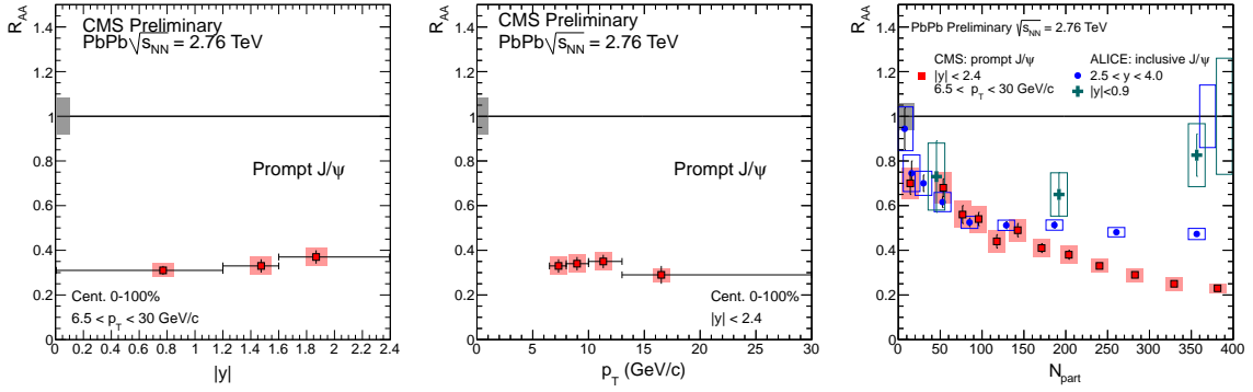
Figure 3. The R_{AA} of prompt J/\psi with respect to rapidity ( left ), p_T ( center ) and centrality ( right ) are presented. Inclusive J/\psi measurement by ALICE ( blue, green markers ) are compared as a function of centrality.
