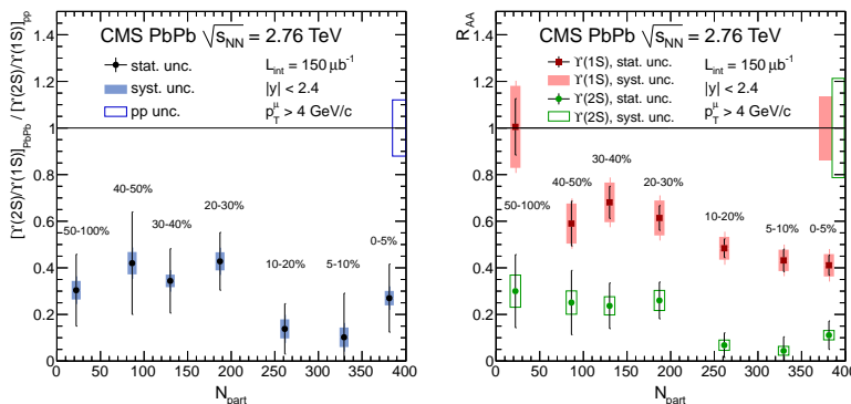
Figure 2. The double ratio ( left ) and the R_{AA} ( right ) of the \Upsilon(2S) and \Upsilon(1S) states are presented as a function of number of participants. The uncertainties that are independent from N_{part} are shown by box at unity.
