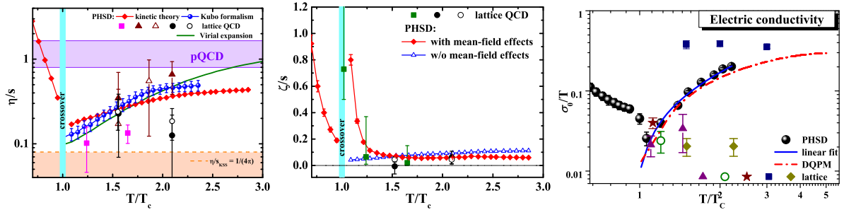
Figure 1. The PHSD results for the shear (left) and bulk (middle) viscosities of partonic and hadronic matter - as well as the electric conductivity (right) - as functions of temperature T/T_c .
