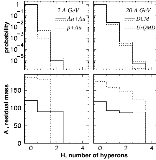
Figure 4. Formation probability of strange spectator residuals (top), and their mean mass numbers (bottom) versus the number of captured \Lambda hyperons (H), calculated with DCM and UrQMD model for p + Au and Au + Au collisions with energy of 2 GeV (left), and 20 GeV per nucleon (right).
