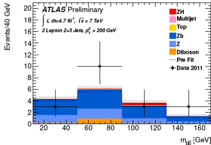
(e) p_T^Z > 200 \text{ GeV}
