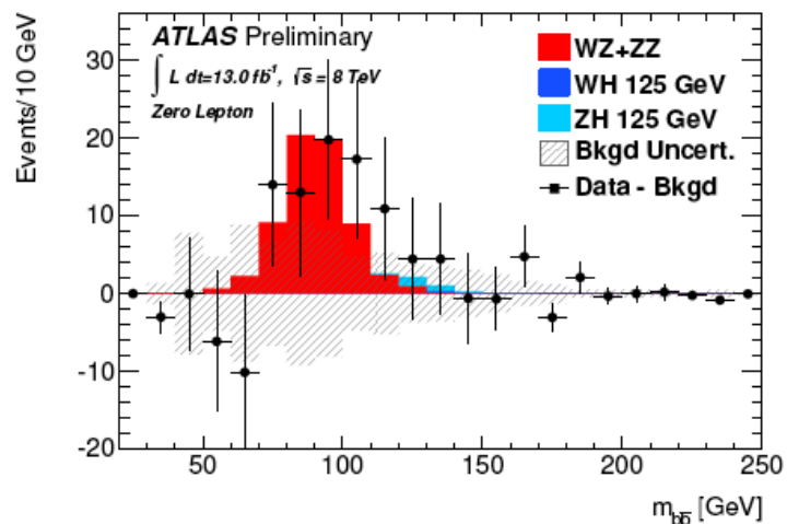
(a) Zero Lepton
