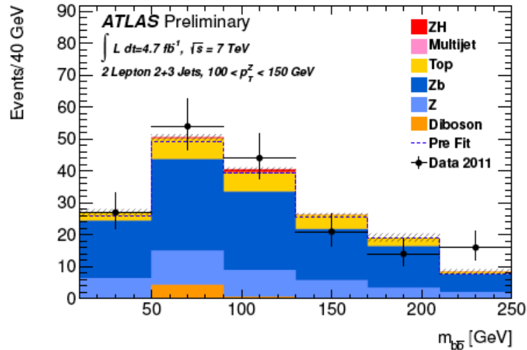
(c) 100 < p_T^Z < 150 \text{ GeV}
