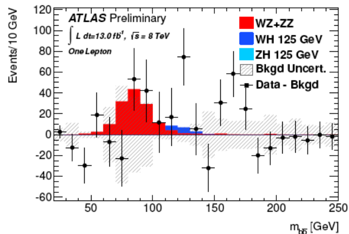
(b) One Lepton
