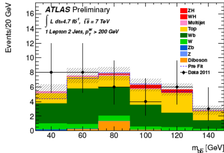
(e) p_T^W > 200 \text{ GeV}
