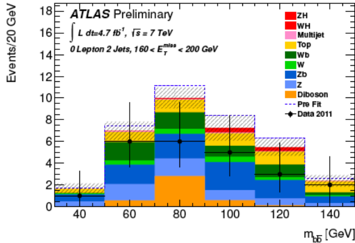
(c) 160 < E_T^{\text{miss}} < 200 \text{ GeV} , 2 jets
