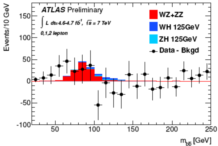
(a) \sqrt{s} = 7 \text{ TeV}
