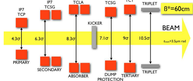
Figure 1: Tight collimator settings for 4 TeV beam energy and \beta^* = 60\text{ cm} .
