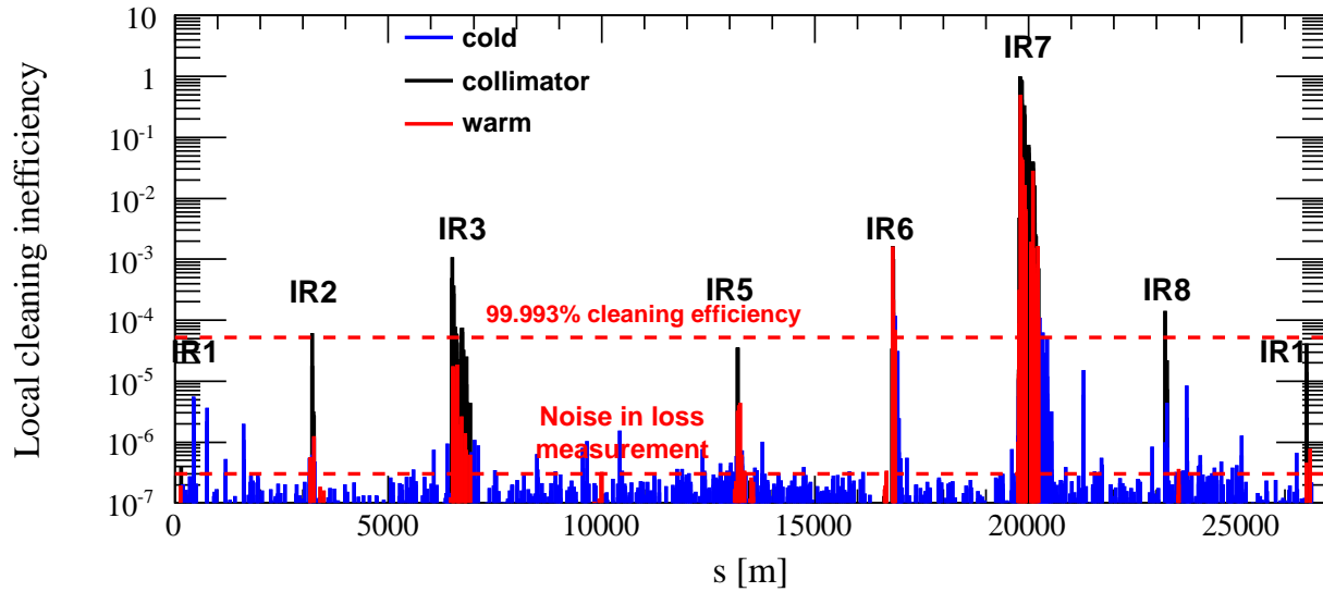
Figure 3: Distribution of the losses in the LHC ring while exciting beam 1 in the horizontal plane.
