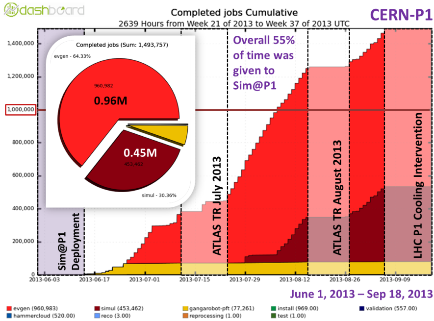
Figure 3. Summary of the cumulative number of successfully completed jobs for the CERN-P1 site during the period of the first 3 production Sim@P1 runs.
