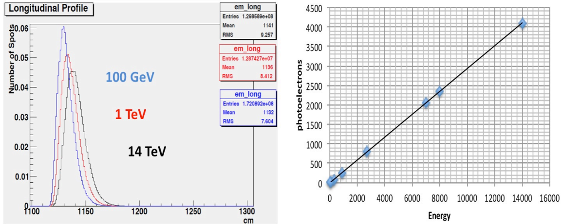
Figure 1. Left plot : Longitudinal Shower Profile produced by HF GFlash for electron with energy 100 GeV (blue), 1 TeV (red) and 14 TeV (black). This plot shows the capability of HF GFlash to handle very high energy particle simulation. Right plot: HF GFlash has linear energy response for electron with energy from 50 GeV to 14 TeV
