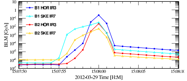
Figure 7: Loss distribution as a function of time for primary collimator in IR3 and primary skew collimator in IR7 using the slow logging of the BLM data (1 Hz).
