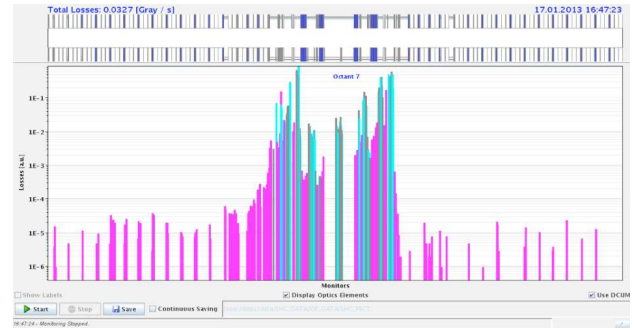
Figure 5: Distribution of the losses in IR7 during an alignment problem.
