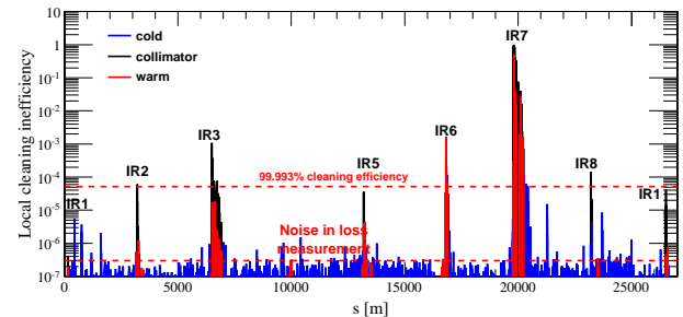
Figure 1: Distribution of the losses in the LHC ring while exciting Beam 1 in the horizontal plane.
