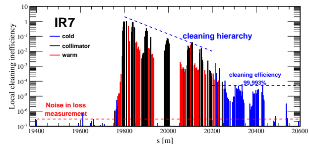
Figure 2: Distribution of the losses in the betatron cleaning insertion (IR7) while exciting Beam 1 in the horizontal plane.
