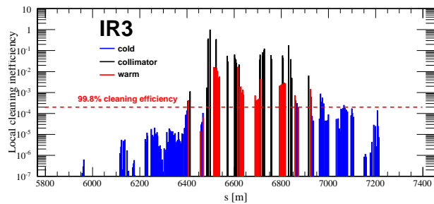
Figure 4: Distribution of the losses in the momentum cleaning insertion (IR3) for a negative off-momentum loss map.
