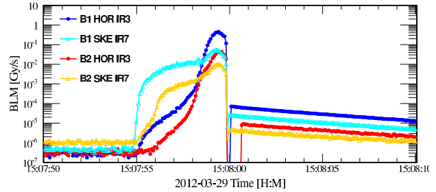
Figure 8: Loss distribution as a function of time for primary collimator in IR3 and primary skew collimator in IR7 using the fast logging of the BLM data (12 Hz).
