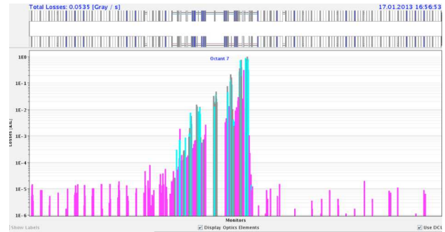
Figure 6: Distribution of the losses in IR7 after the correction of the alignment problem at the TCL.A6L7.B2.
