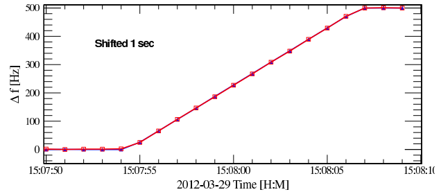
Figure 9: RF frequency change as a function of time.
