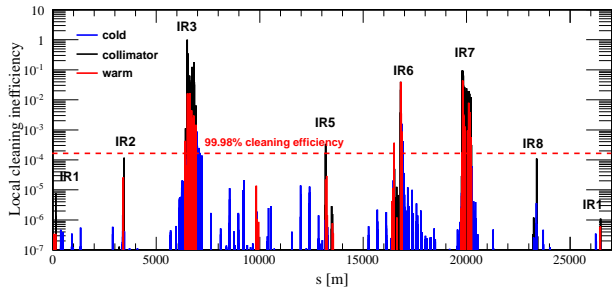
Figure 3: Distribution of the losses in the LHC ring for a negative off-momentum loss map.
