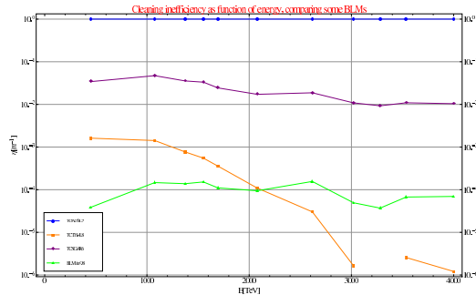
Figure 10: Leakage to Q8 and tertiary collimators during energy ramp cycle [11].
