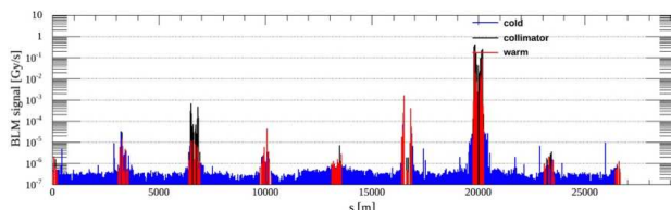
Figure 11: Losses during a regular fill on 2012-12-04 18:09:29 along the LHC ring.
