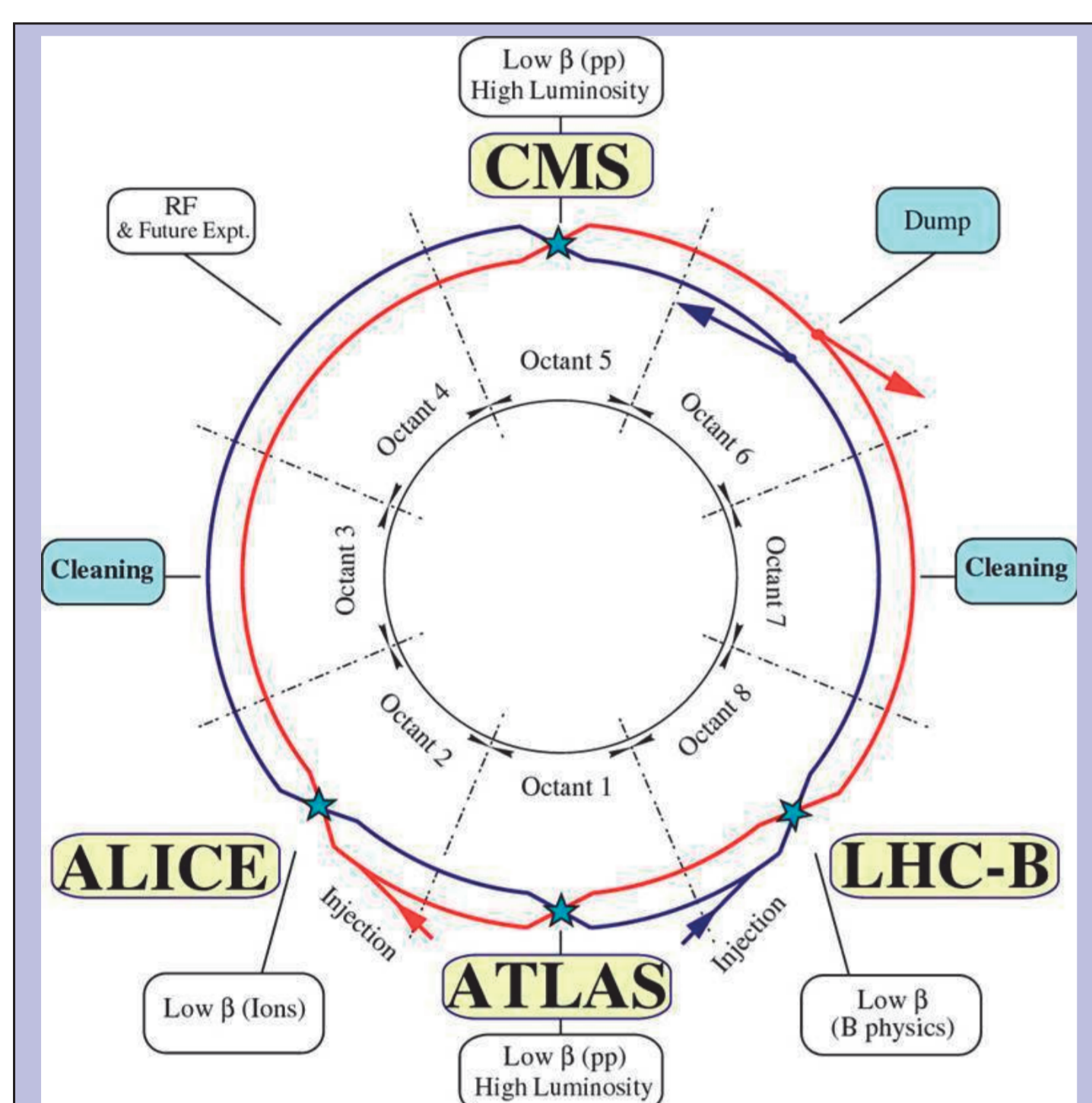
Figure 2: Overview schematic shows the four main experiments and the two ring structure of the LHC [http://lhc-machine-outreach.web.cern.ch].
