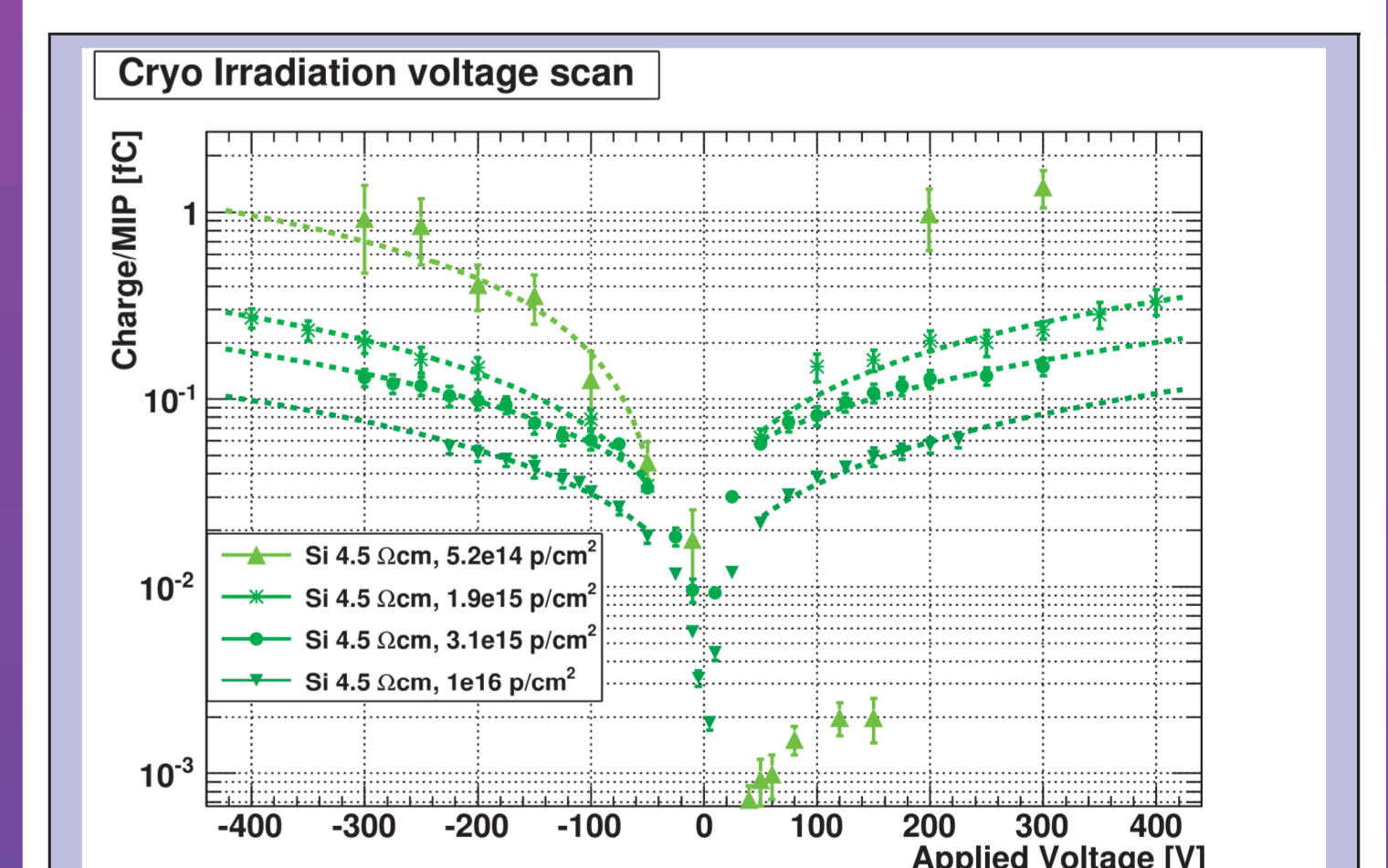
Figure 15: Voltage scan for 4.5 Ωcm silicon.
