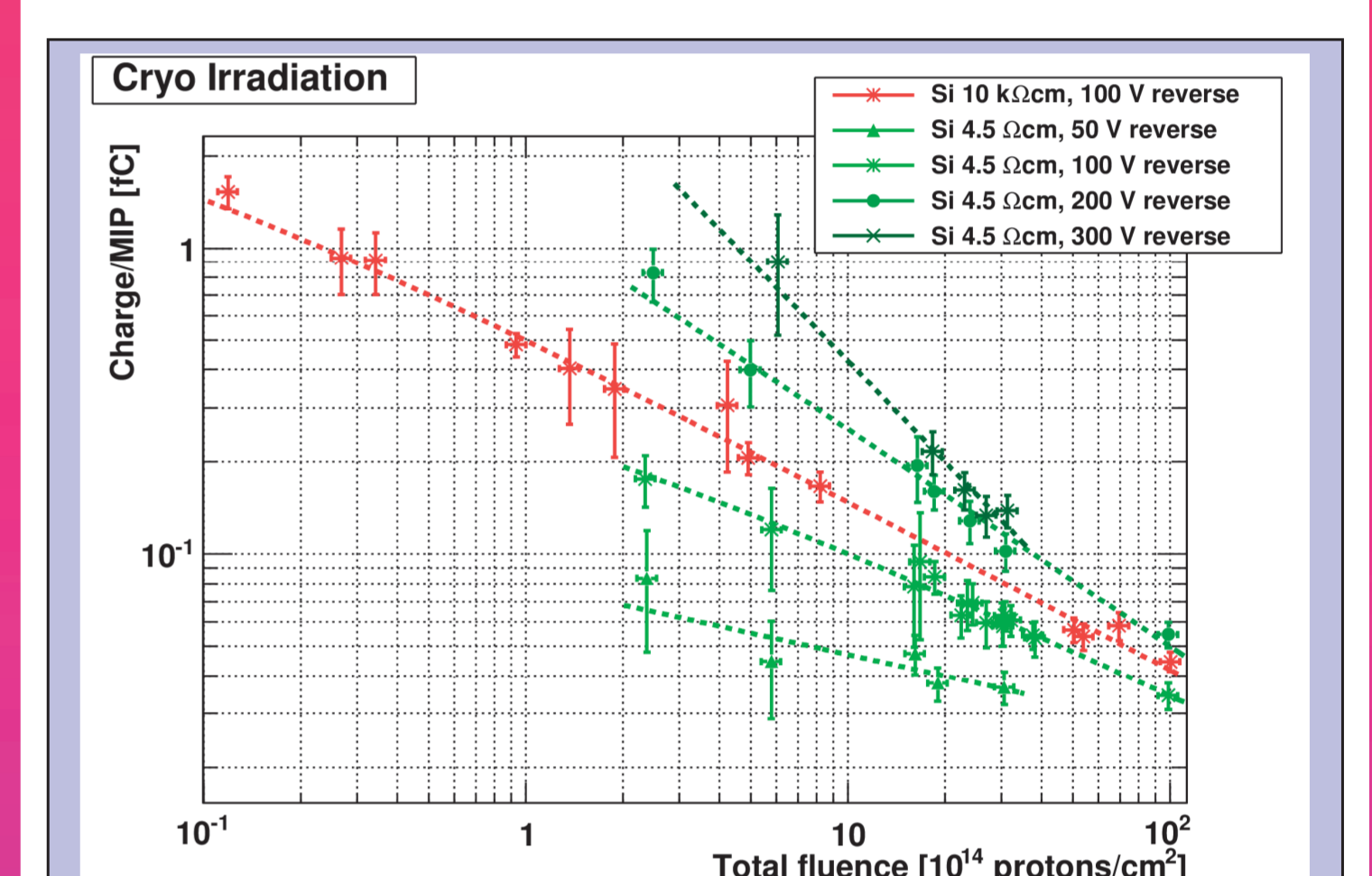
Figure 13: Dependence of the charge collected in Si detectors with a resistivity 4.5 Ωcm on fluence.
