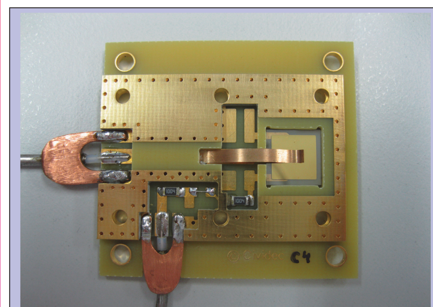
Figure 9: Holder for DC readout from Cividec.
