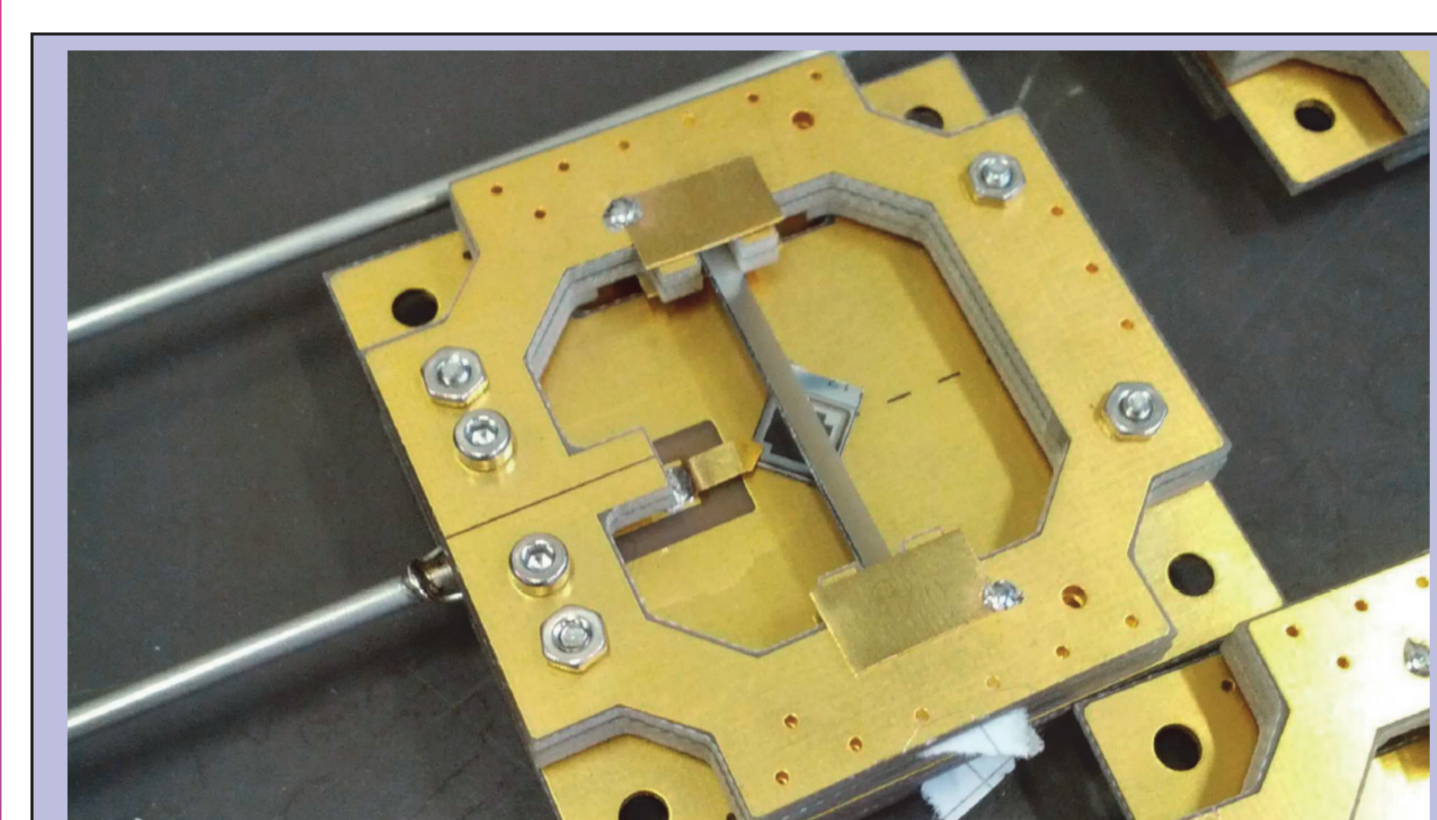
Figure 10: Holder for TCT measurements.
