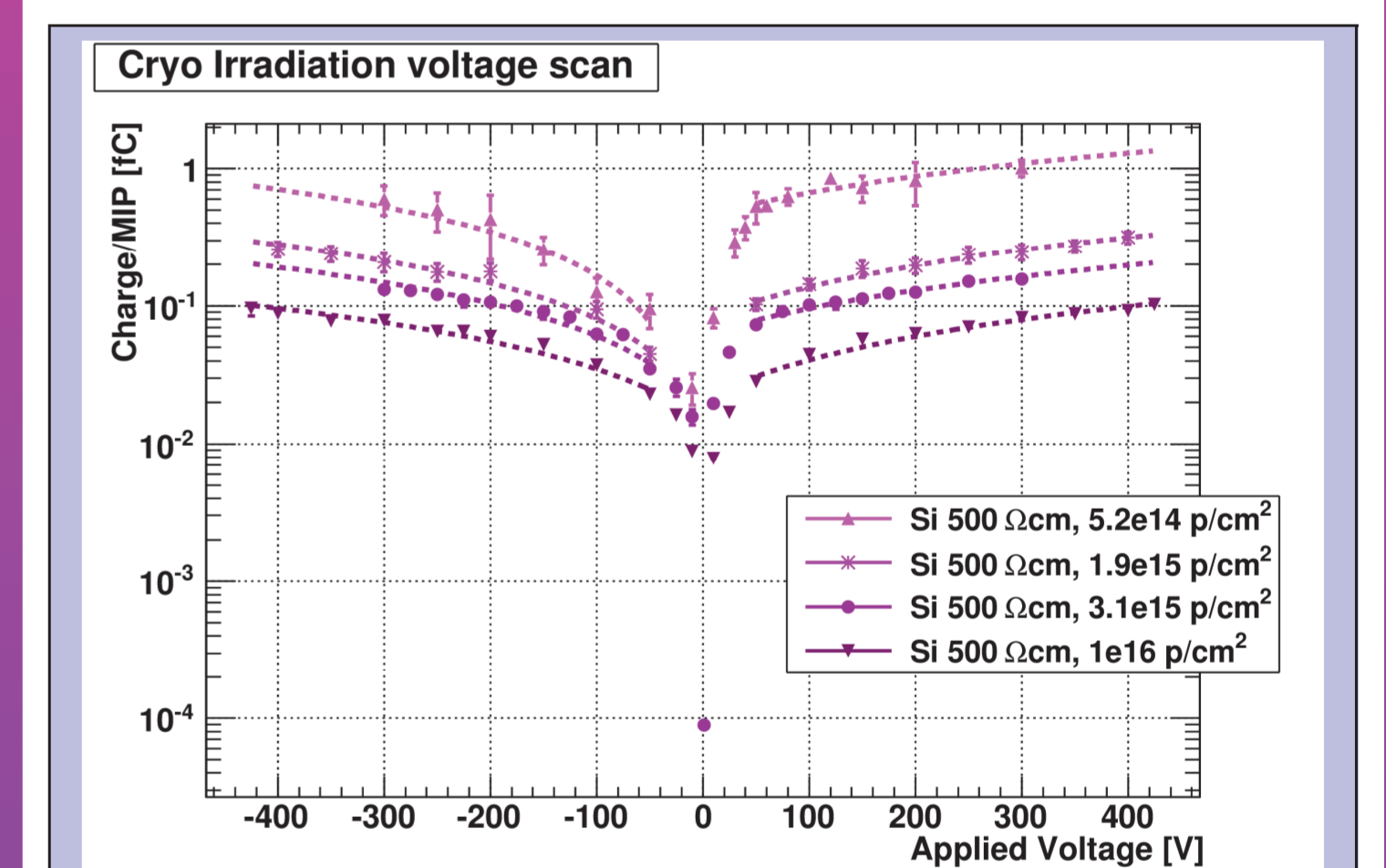
Figure 14: Voltage scan for 500 Ωcm silicon.
