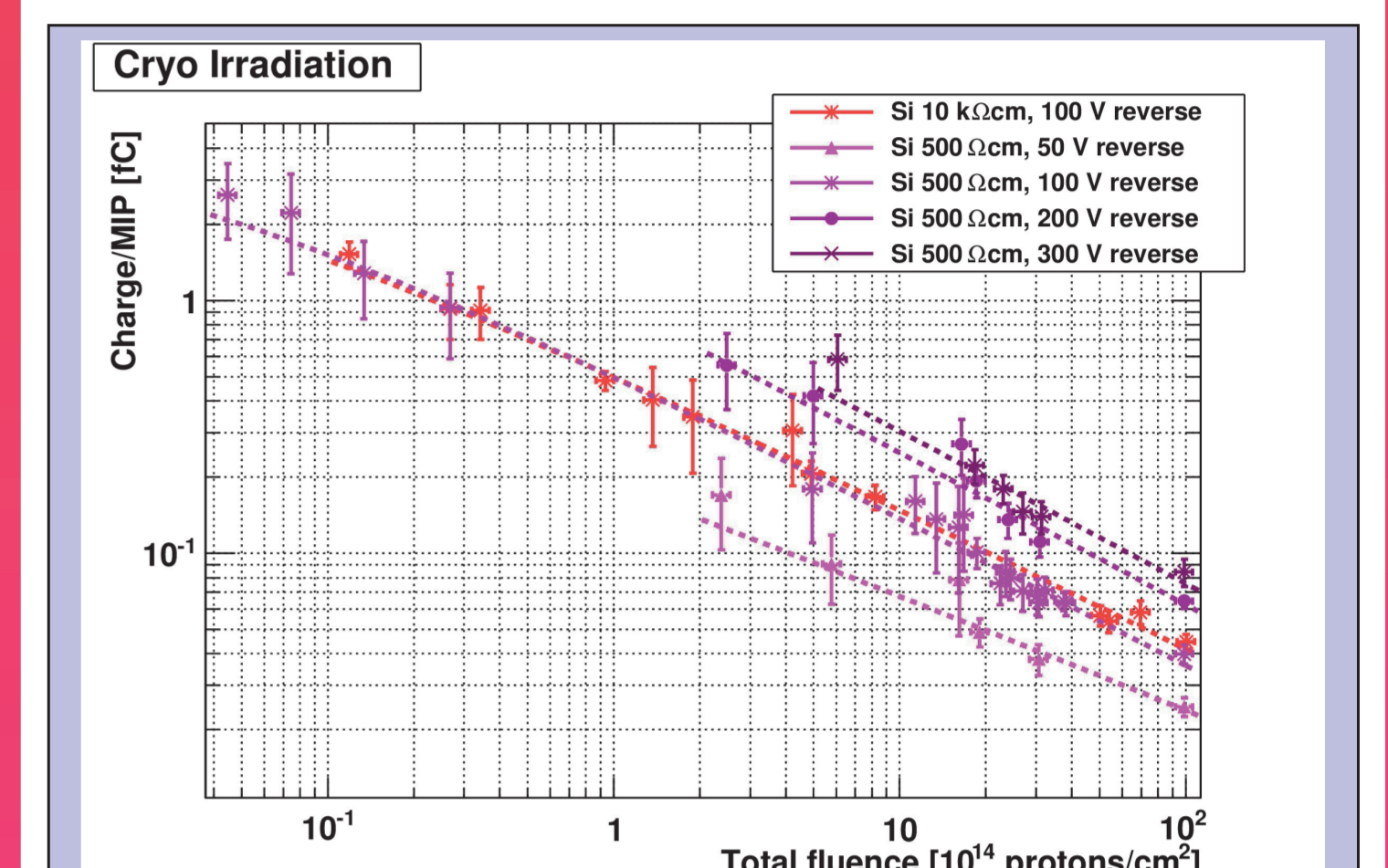
Figure 12: Dependence of the charge collected in Si detectors with a resistivity 500 Ωcm on fluence.
