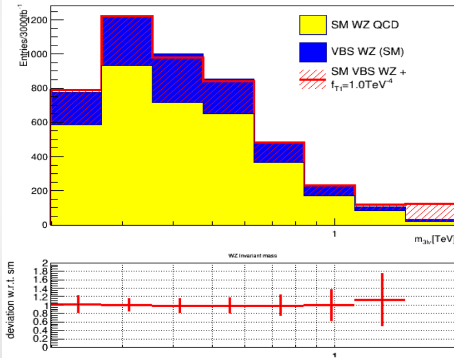
WZ invariant mass
