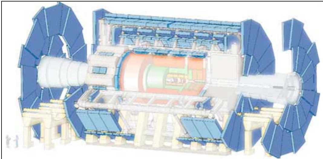
Figure 5 : Muon Chambers
