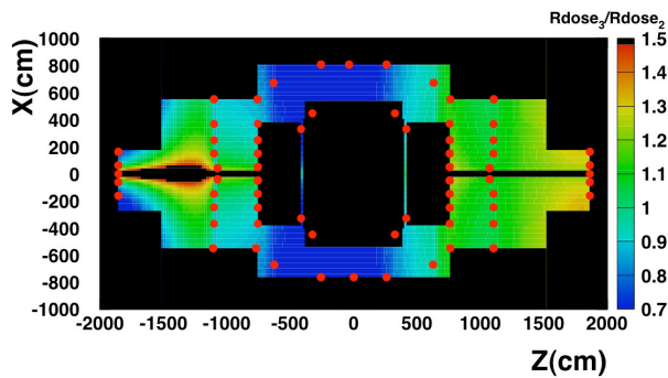
Figure 5: Ratio of ionizing radiation dose rates before/after installation of shielding surrounding the incoming proton focusing quadrupole magnets. Protons are incident from the left. The red spots indicate locations of TLDs used in the measurements. Sensitive electronics are located in the “central corners” of the collision hall, near z = \pm 700 cm.
