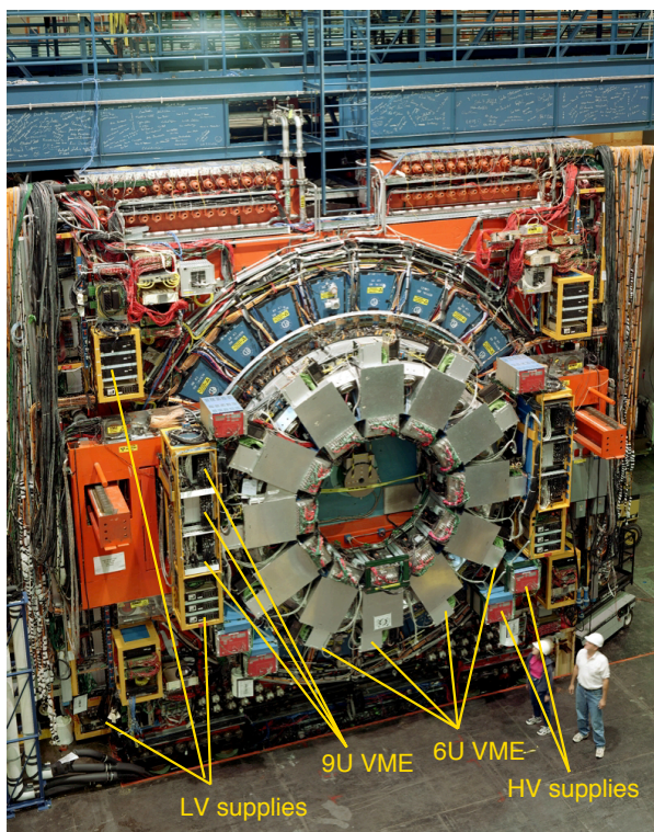
Figure 1: Photograph of the CDF detector. Some of the electronics found to be sensitive to radiation are indicated. For reference, protons are incident into the page.
