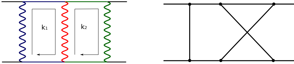
Figure 1. Left: The planar double box with loop momenta as used for the loop-by-loop presentation. Right: The non-planar double box.
