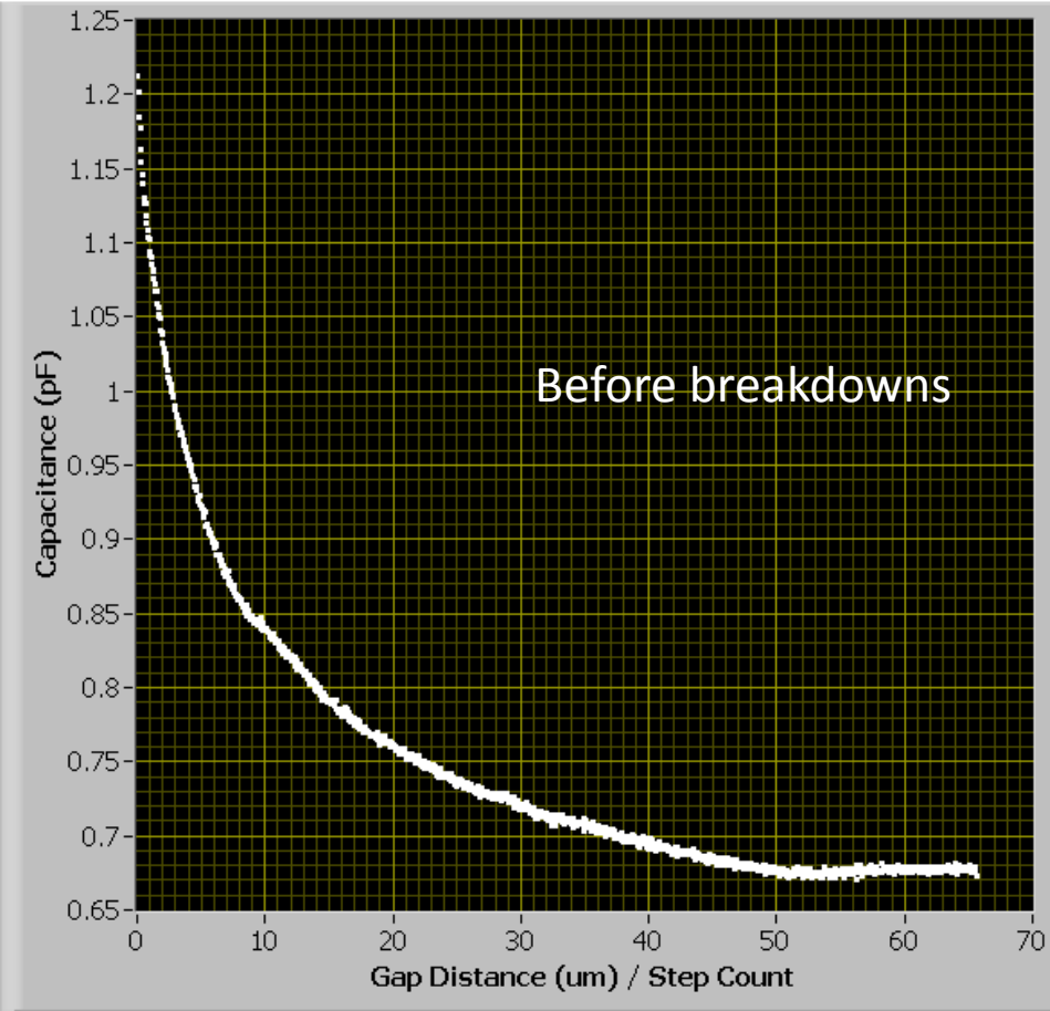
Capacitance versus Position
