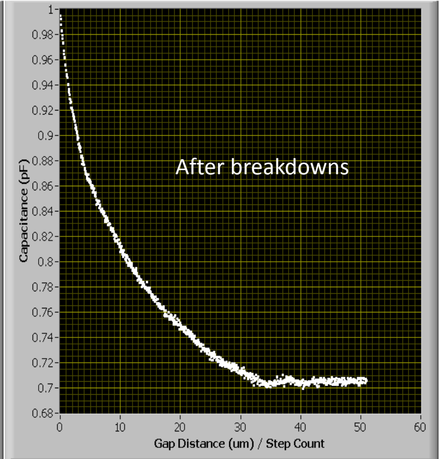
Capacitance versus Position
