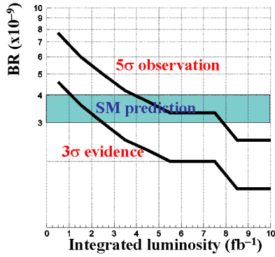
FIG. 3: Luminosity needed for the observation of a given branching ratio of B_s^0 \rightarrow \mu^+ \mu^- at 3\sigma (lower line) and 5\sigma (upper line) level.
