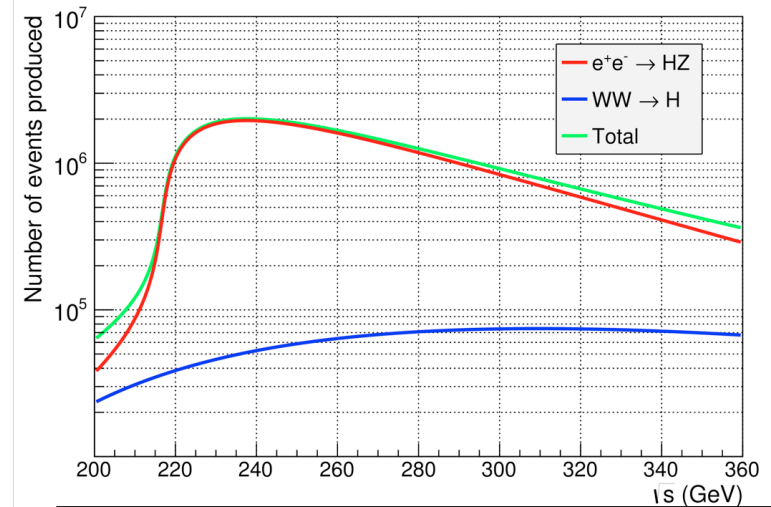
N Higgs boson produced in 5-year running program
