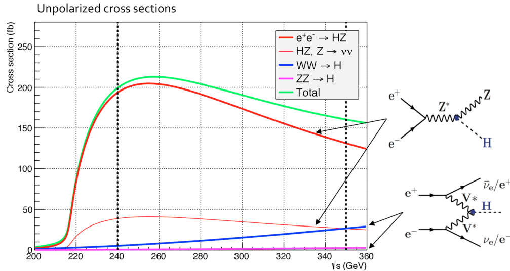
Higgs production cross section in un-polarized e+e- collisions (from the HZHA generator)
