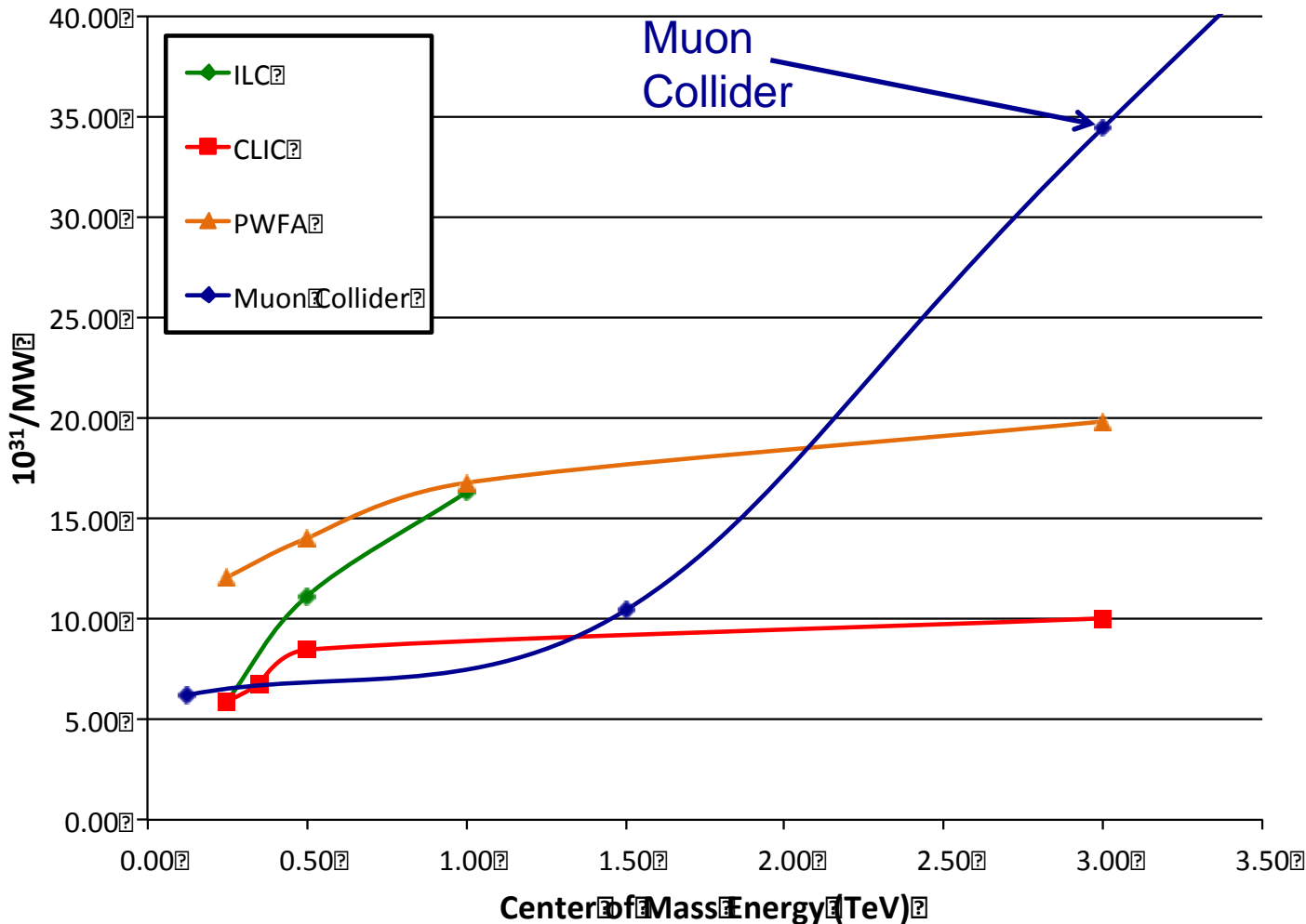
Lepton Colliders Figure of Merit: Luminosity/Wall Power
