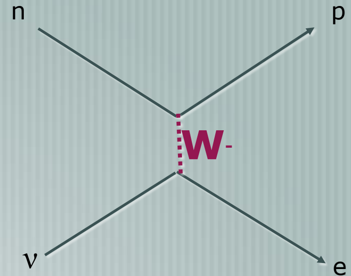
Glashow model
