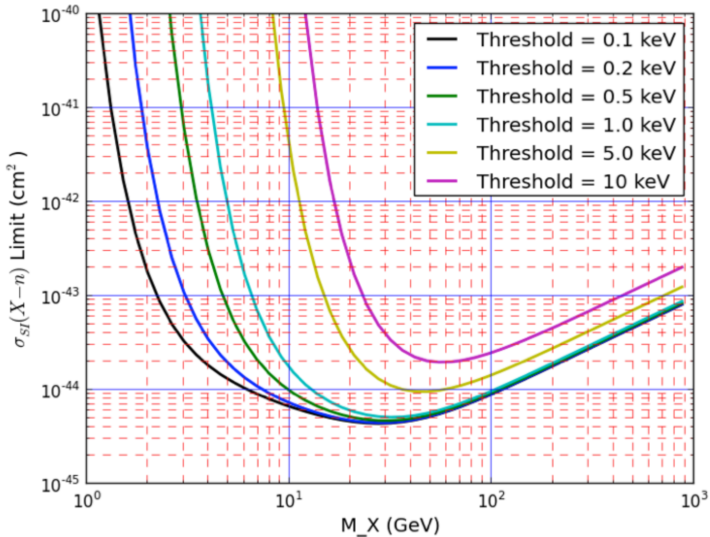
Gold target, 365 kg-day exposure
