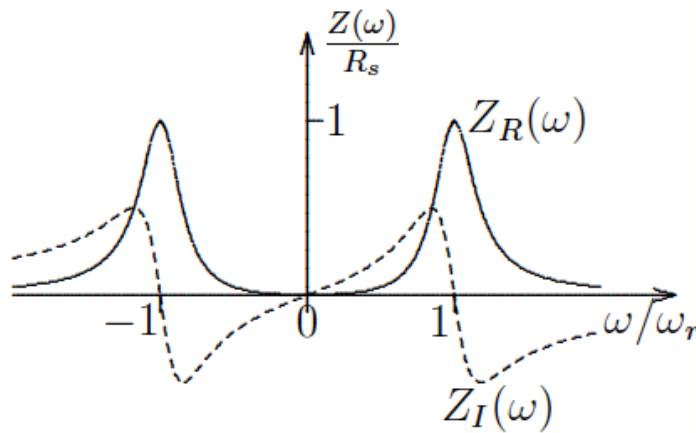
Impedance
