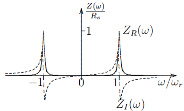
Impedance
