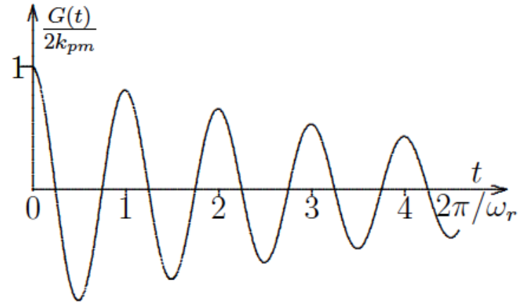
Green function
