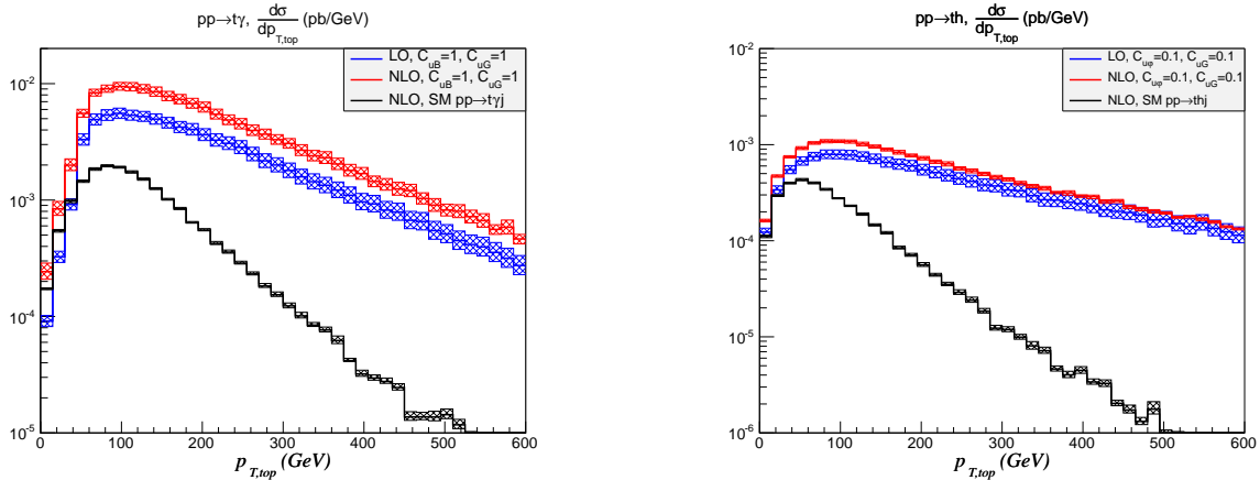
Figure 4. p_T distribution of the top quark in pp \rightarrow t\gamma (left), and in pp \rightarrow th (right). The SM background is from t\gamma j (left) and thj production (right).
