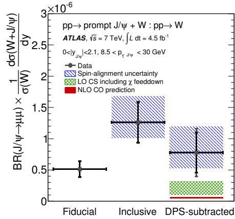
Figure 6. The W +prompt J/\psi to inclusive W production cross-section ratio [12].
