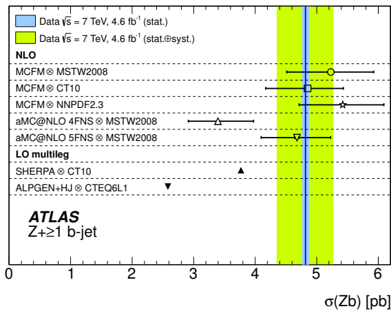
Figure 3. Cross-section for Z+\geq 1b -jet and comparison with theoretical predictions [10].
