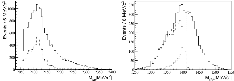
Figure 2. Left: \Lambda p invariant mass for the inclusive \Lambda p selection (continuous line) and for events with an extra \pi^- detected (dashed line). Right: \Sigma^0 \pi^0 invariant mass (dashed and pointed line represent the at-rest and in-flight components, respectively).
