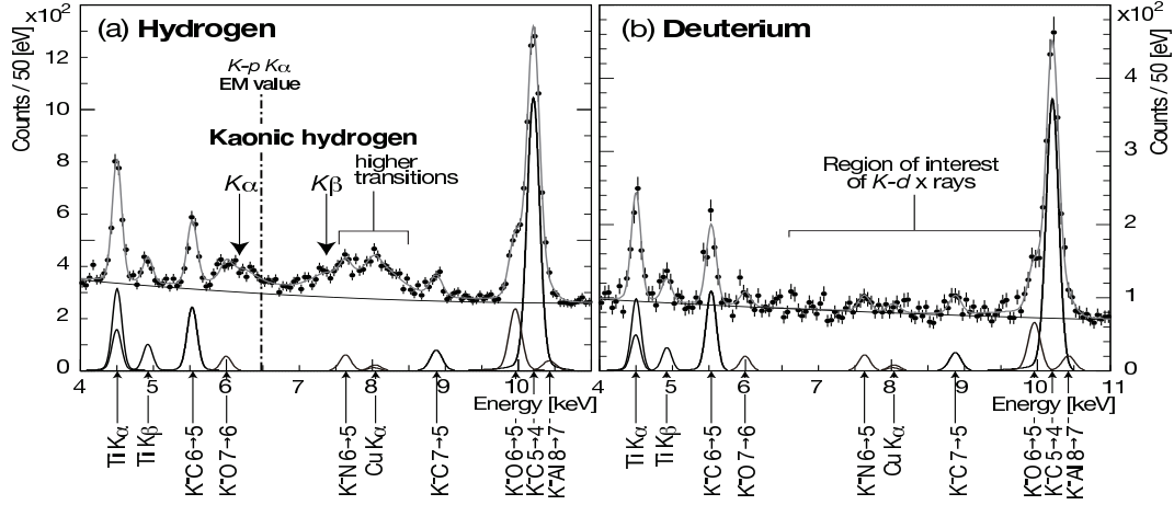
Figure 1. Global fit of the X-ray spectra from kaonic hydrogen (a) and kaonic deuterium (b). The dot-dashed vertical line indicates the EM energy of the kaonic-hydrogen K\alpha X-ray.
