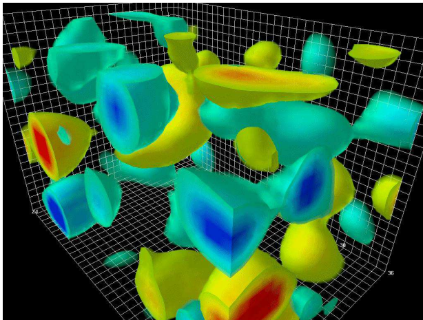
Lattice simulation of fluctuations in the local topological charge [Leinweber]
