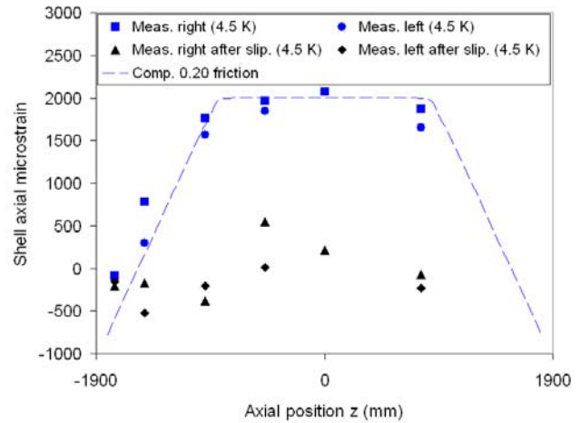
Figure 10. Shell axial strain versus length for LRS01 at 4.5 K, before and after the loss of strain.
