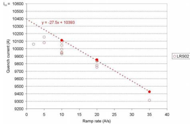
Figure 12. Quench currents in LRS02. The fit is to the highest currents at each ramp rate (solid symbols).
