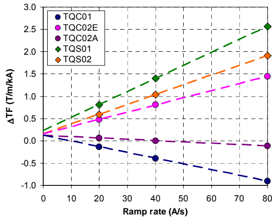
Figure 7. Measurement of the eddy current effect on the transfer function at a gradient of 45 T/m.
